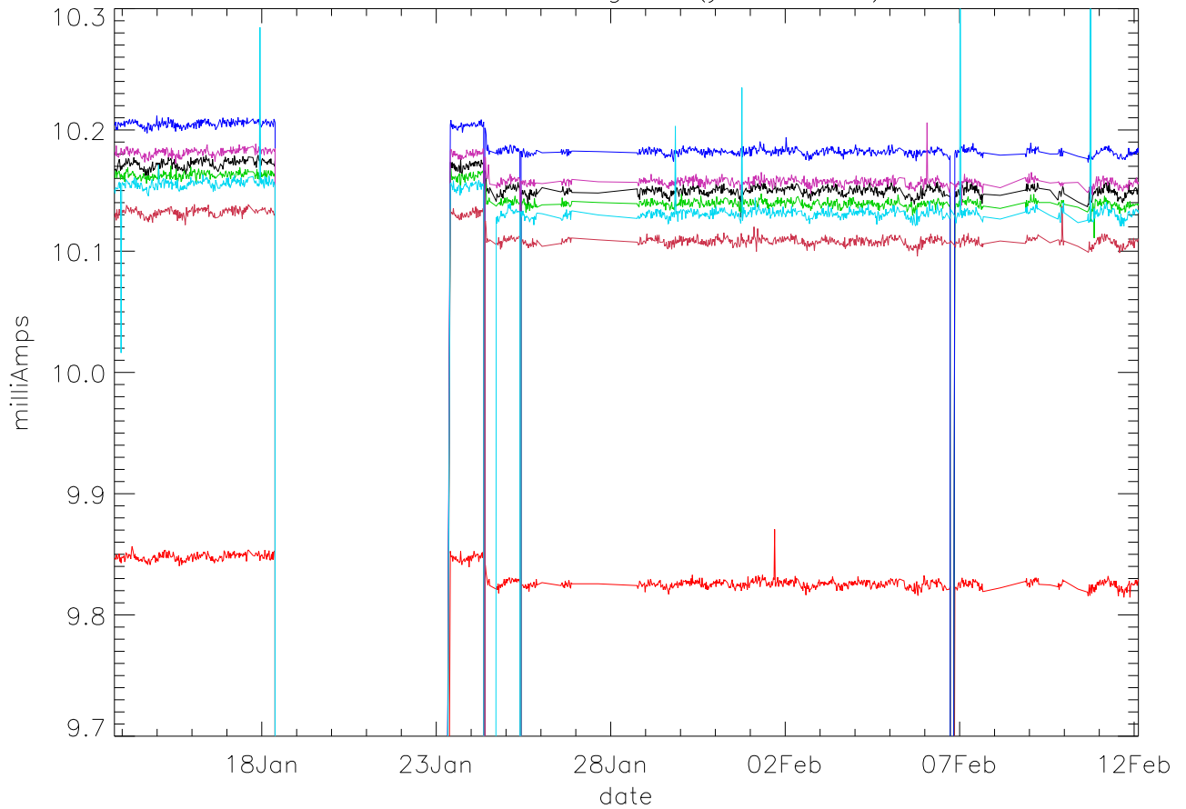
Id:Drain Current. stage 2 (year 2012) PoIB
