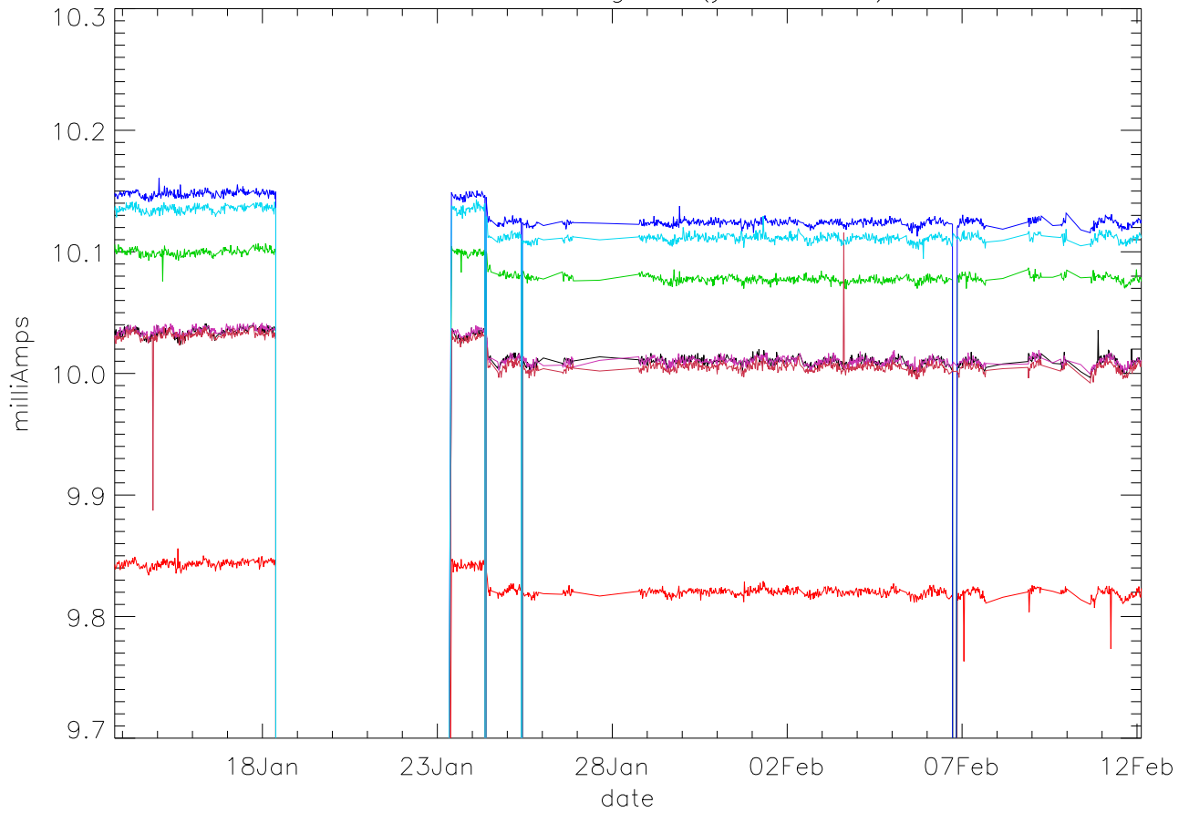
Id:Drain Current. stage 2 (year 2012) PoIB
