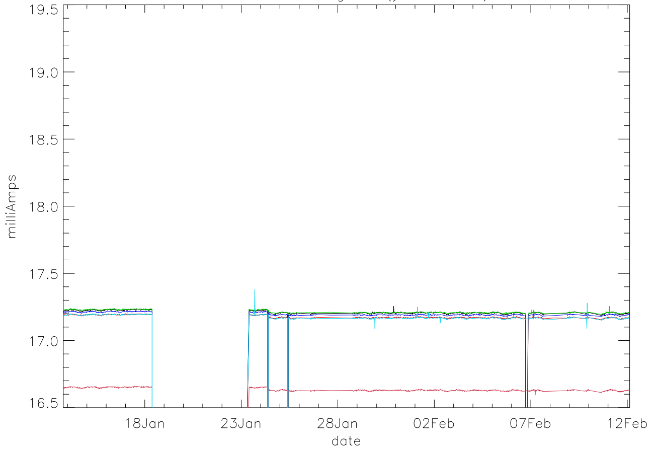
Id:Drain Current. stage 3 (year 2012) PoIB
