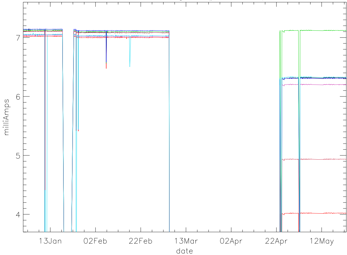
Id:Drain Current. stage 1 (year 2012) PoIB
