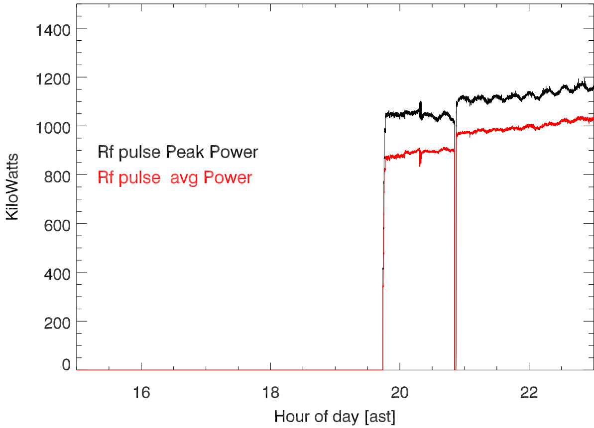
20180117 t1193 430tx power (dome) vs hour of day
