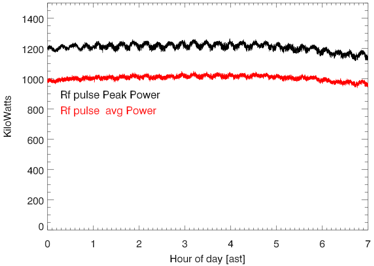
20180119 t1193 430tx power (dome) vs hour of day
