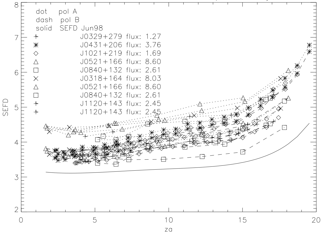
SEFD vs za LBN, 1400 Mhz, Jun/Jul 00 day
