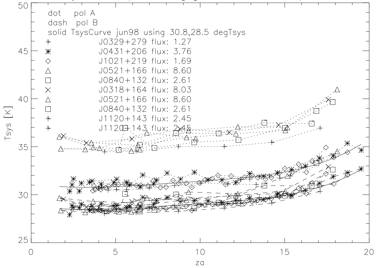
System temp Off src [K], lbn 1400 Mhz, Jun/Jul00
