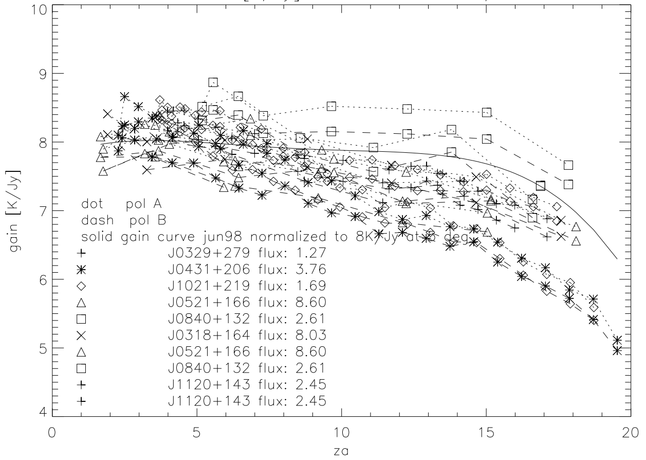
Gain vs za [K/Jy], Ibn 1400 Mhz, Jun/Jul00
