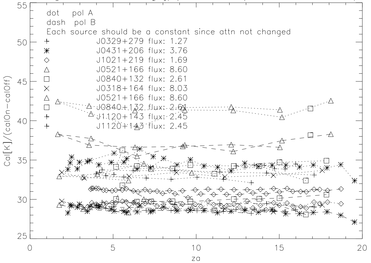
cal Scaling factor vs za: \text{cal}[K]/(\text{calOn}-\text{calOff}) , lbn 1400 Mhz, Jun/Jul00
