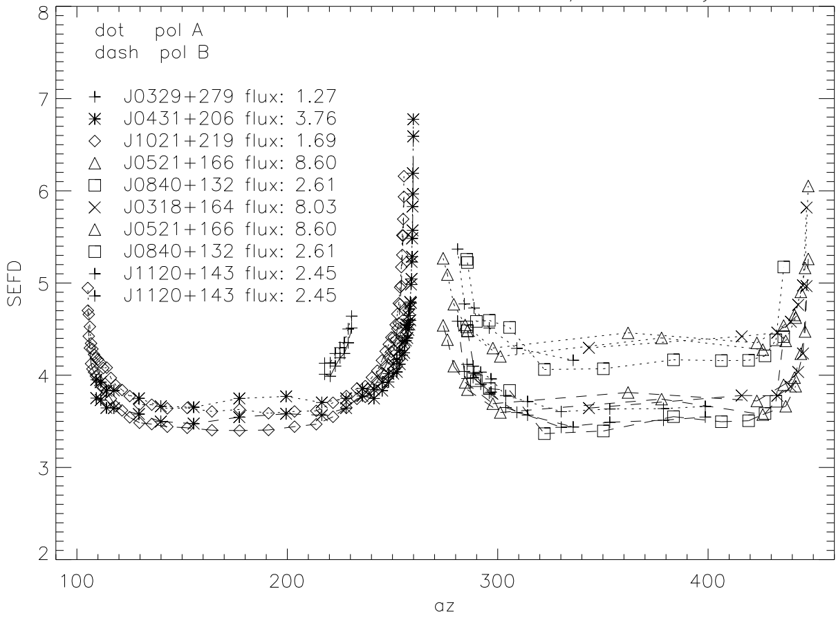
SEFD vs az LBN, 1400 Mhz, Jun/Jul 00 day
