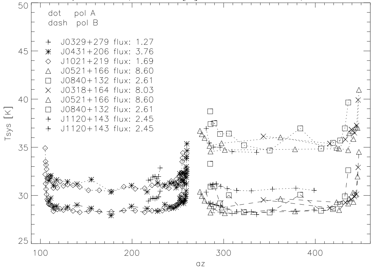
System temp Off src [K], lbn 1400 Mhz, Jun/Jul00
