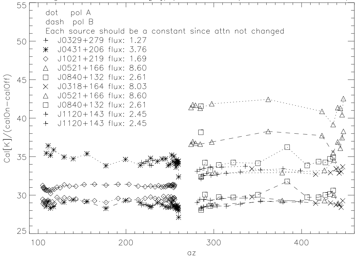
cal Scaling factor vs az: \text{cal}[K]/(\text{calOn}-\text{calOff}) , Ibn 1400 Mhz, Jun/Jul00
