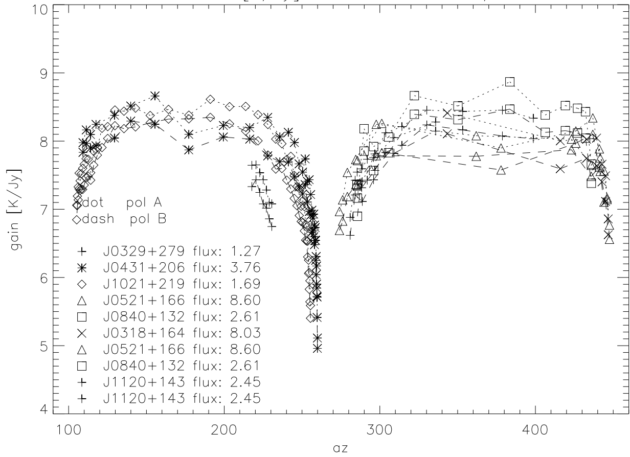
Gain vs az [K/Jy], Ibn 1400 Mhz, Jun/Jul00
