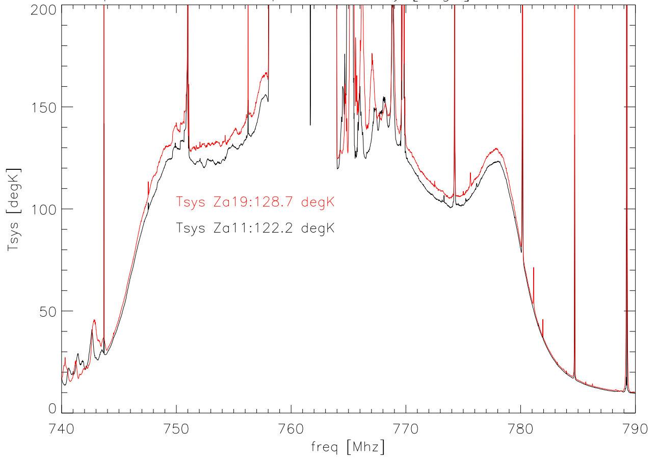
08apr09 800MhzRcv Spectral Density [degK] at za=11,za=19
