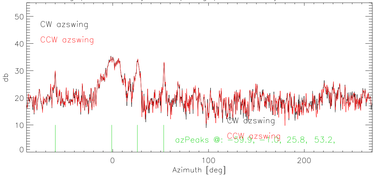
chan63 Video PkValue vs azimuth (rbw=21Khz)
