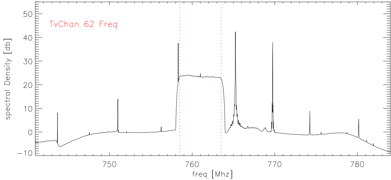
AvgSpectralDensity Chn62/ AvgSpectralDensity vs Azimuth
