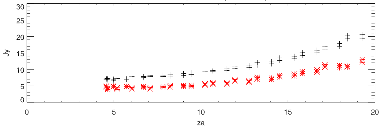
SEFD Vs Za (no cal dependence)
