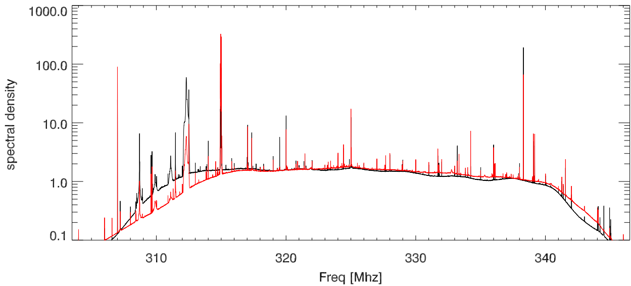
max hold Spectra from 7 cross patterns
