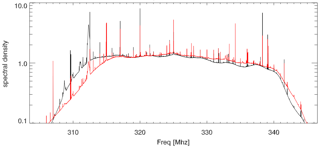
median Spectra from 7 cross patterns
