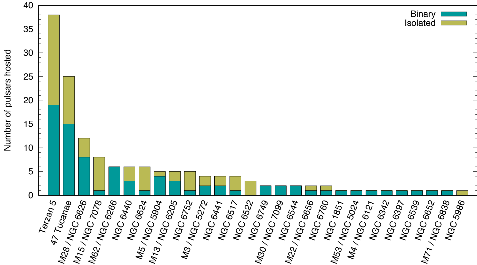
150 pulsars in 28 clusters
