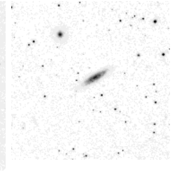
NGC 3972
