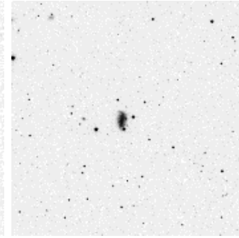
NGC 3782
