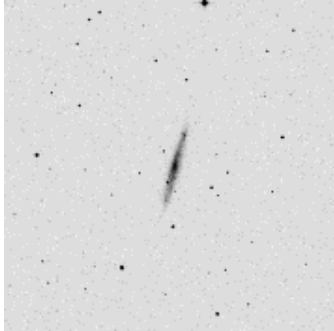
NGC 4183
