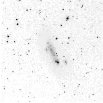
NGC 2366
