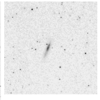
NGC 4758
