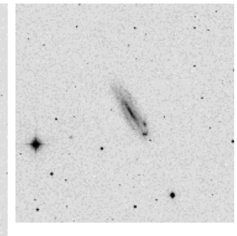
NGC 4178
