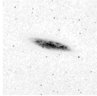
NGC 3556
