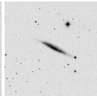
NGC 4157
