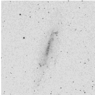
NGC 4236
