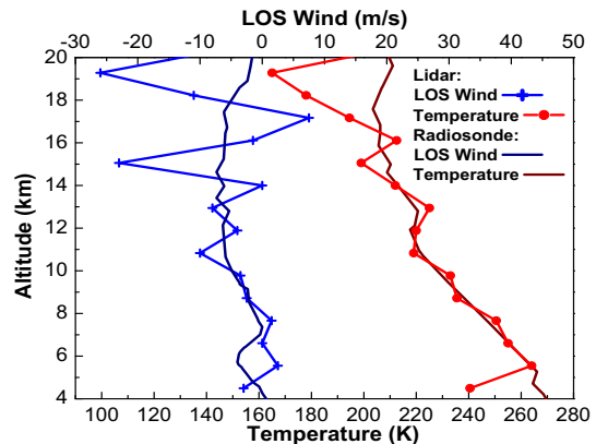
Figure 3. Retrieved LOS wind and temperature on 16 October 2008. The integration time \Delta t is 30 min and the vertical resolution \Delta z is 1 km. The wind and temperature errors are about \pm 1.1 m/s and \pm 2.2 K at 9.8 km.
