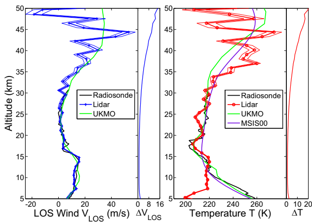
Figure 4. LOS wind and temperature measured on 9 January 2009 at Fort Collins, CO. Radiosonde and model winds are projected to LOS. \Delta z = 1 km and \Delta t = 60 min.
