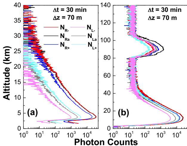
Figure 2. Raw lidar data profiles obtained on 16 October 2008 with two PMTs (a) and on 11 December 2008 with one PMT (b). Vertical resolution is \Delta z = 75 \times \cos(20^\circ) = 70 m.
