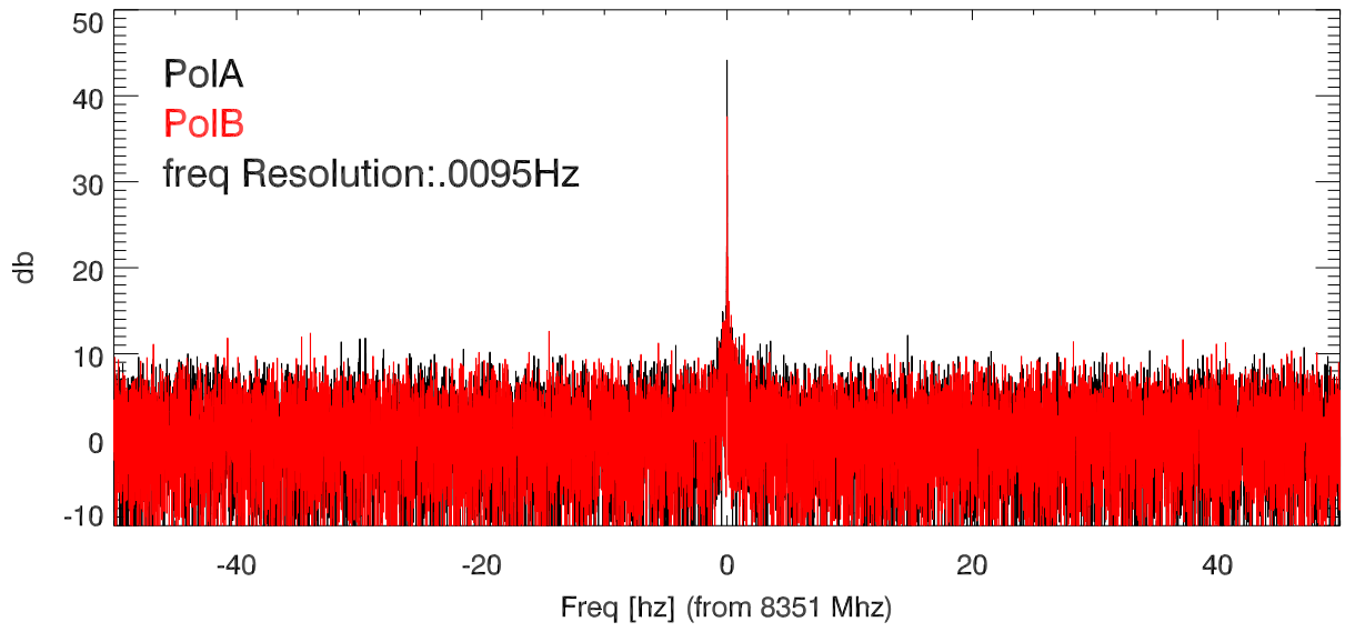
09apr14 xband spectrum. xmt 8351 Mhz from helix in control room
