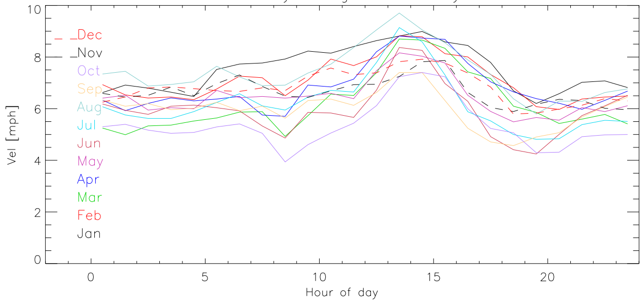
2014 Monthly average wind velocity vs hour
