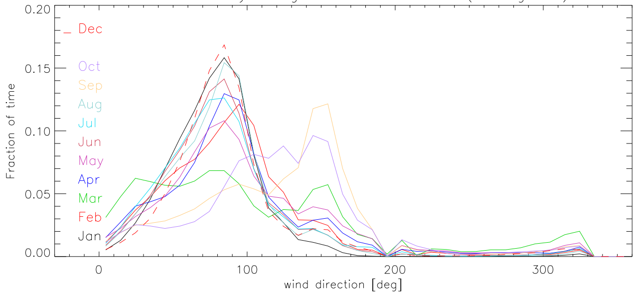
2013 Monthly histogram of wind direction (10 deg bins)
