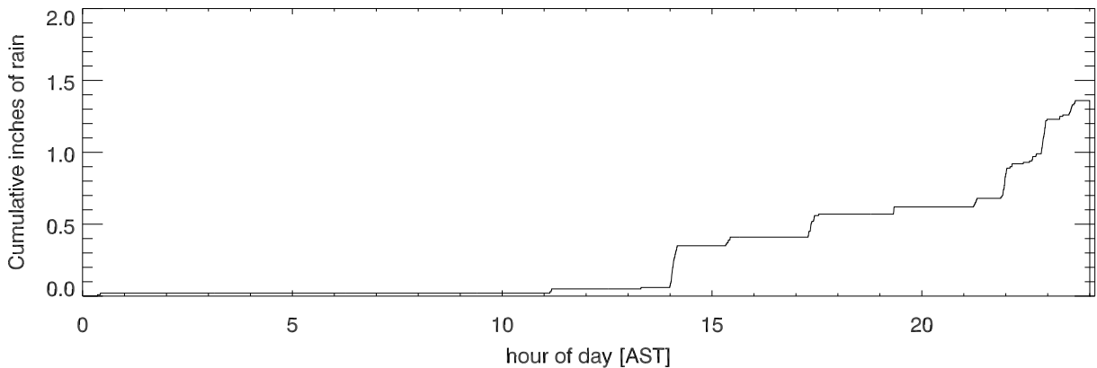
cumulative rain for 19sep17
