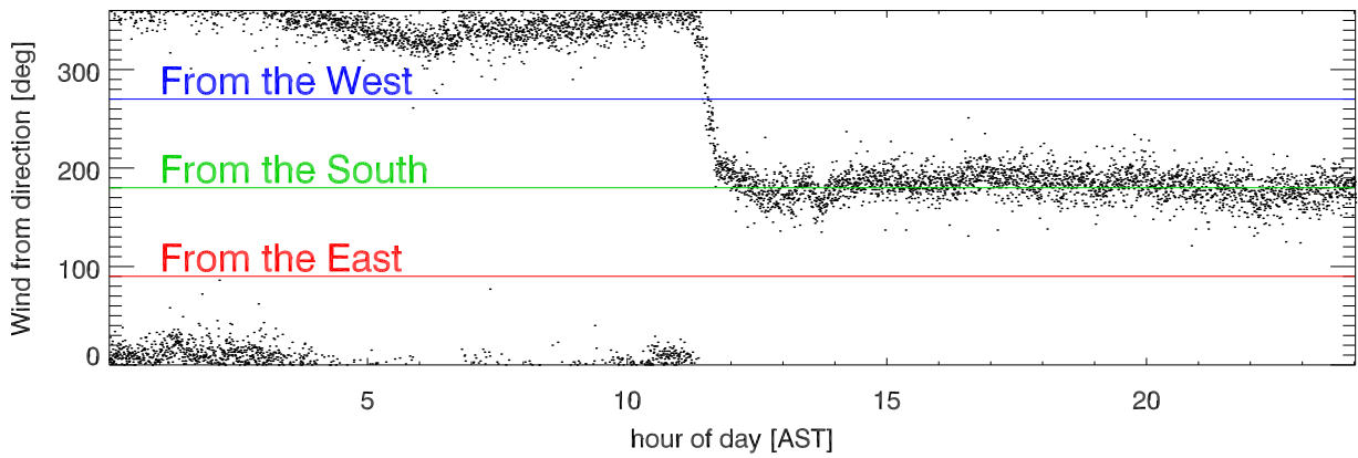
Wind direction for 20sep17
