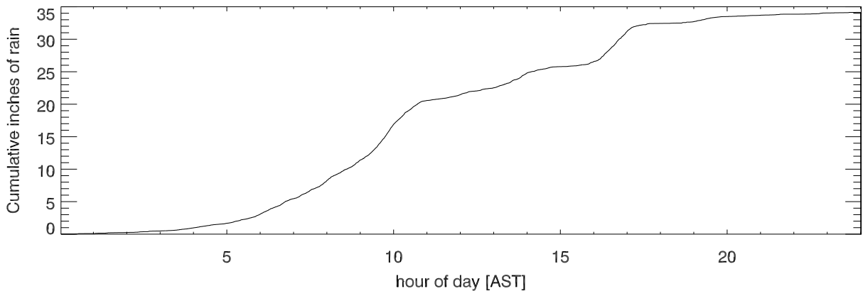
cumulative rain for 20sep17
