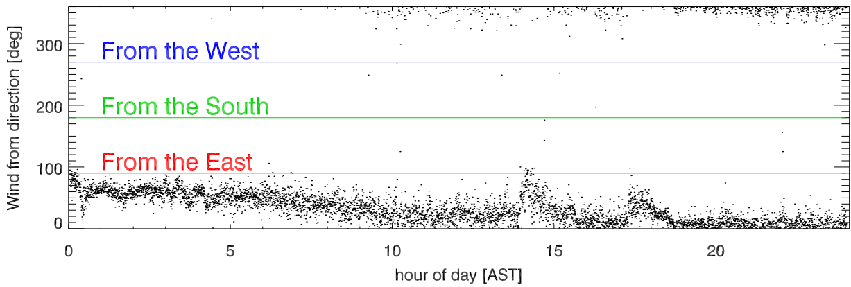
Wind direction for 19sep17
