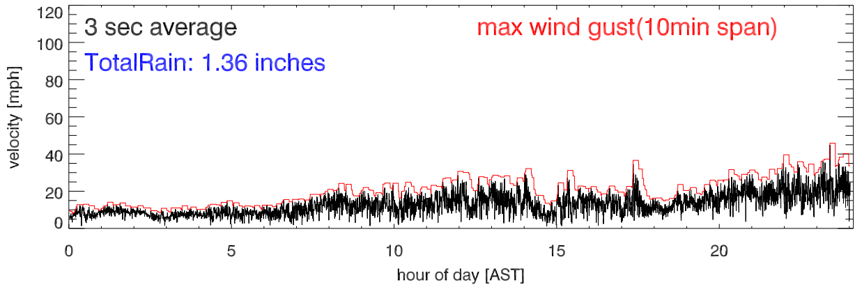
Wind velocity for 19sep17 @:24:01
