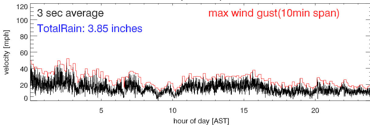
Wind velocity for 21sep17 @:24:01
