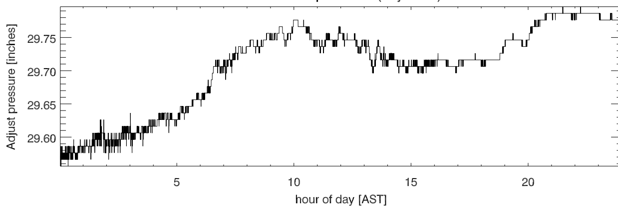
Barometric pressure (adjusted)
