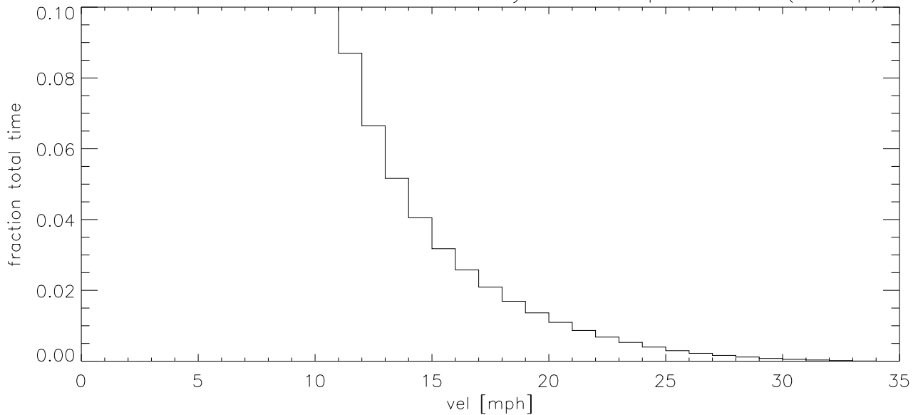
JUL20 Fraction of time wind velocity exceeds specified vel (blowup)
