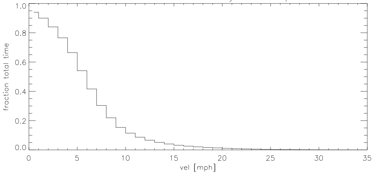
JUL20 Fraction of time wind velocity exceeds specified vel (blowup)
