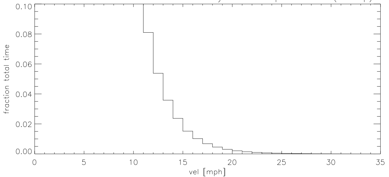
DEC19 Fraction of time wind velocity exceeds specified vel (blowup)
