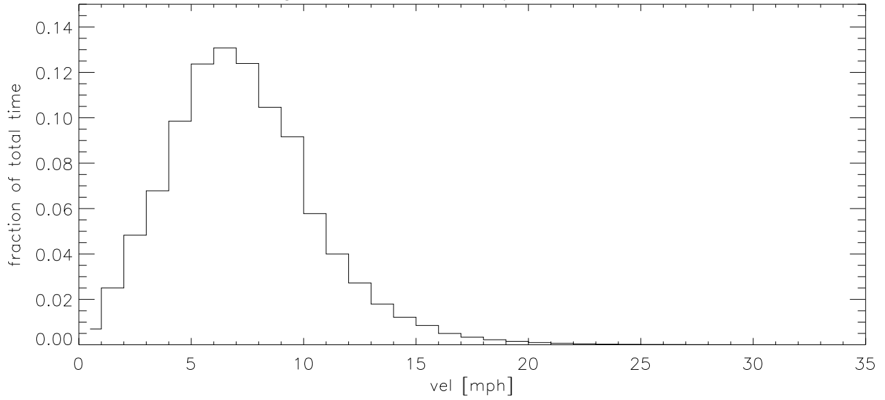
DEC19 Fraction of time wind velocity exceeds specified vel
