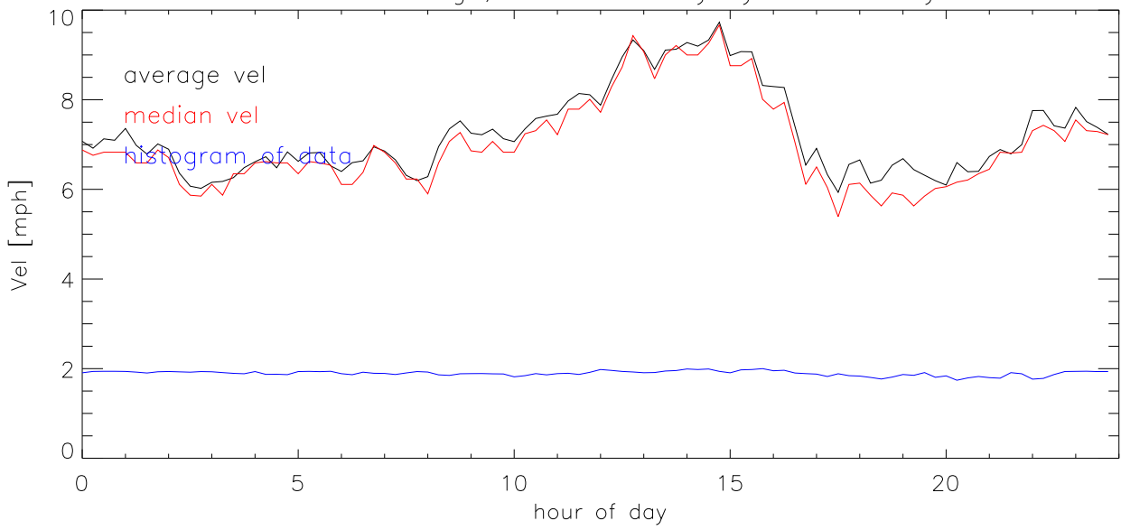
JUL19 Average, median velocity by direction
