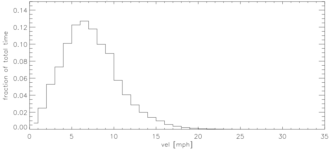
JUL19 Fraction of time wind velocity exceeds specified vel
