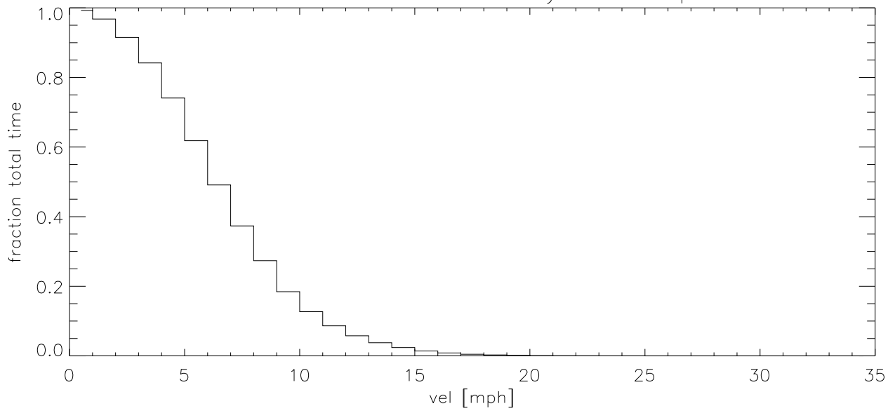
JUL19 Fraction of time wind velocity exceeds specified vel (blowup)
