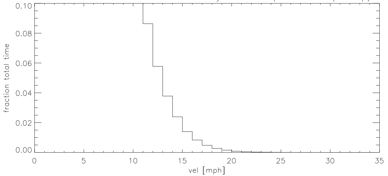
JUL19 Fraction of time wind velocity exceeds specified vel (blowup)
