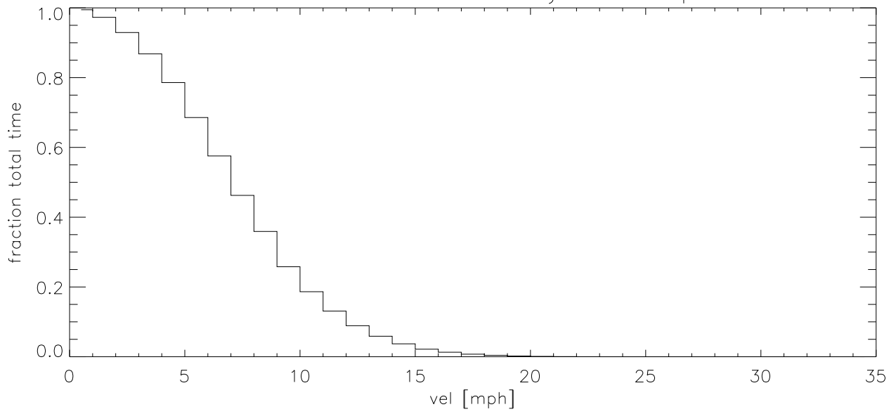
FEB19 Fraction of time wind velocity exceeds specified vel (blowup)
