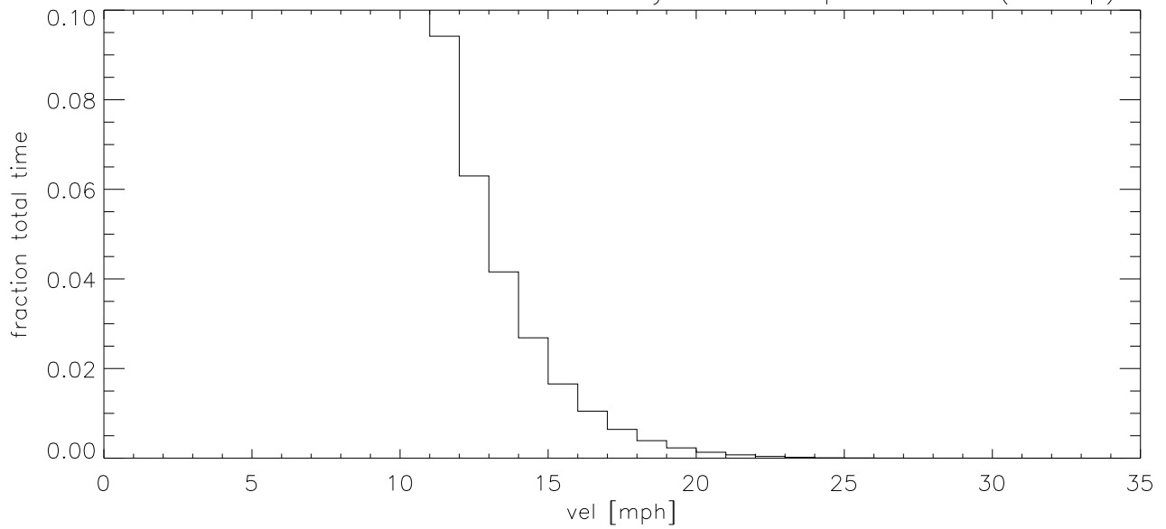
MAY18 Fraction of time wind velocity exceeds specified vel (blowup)
