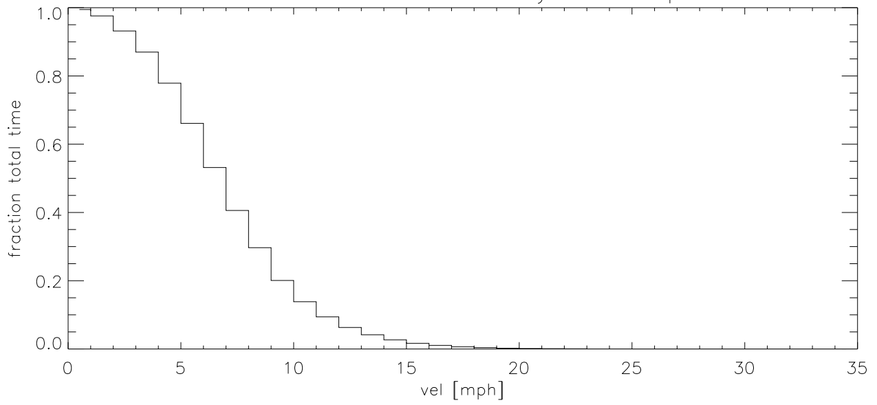
MAY18 Fraction of time wind velocity exceeds specified vel (blowup)
