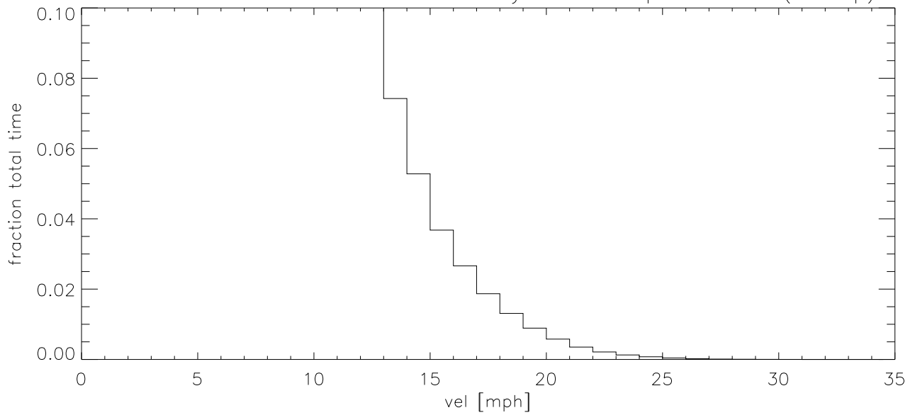
FEB18 Fraction of time wind velocity exceeds specified vel (blowup)
