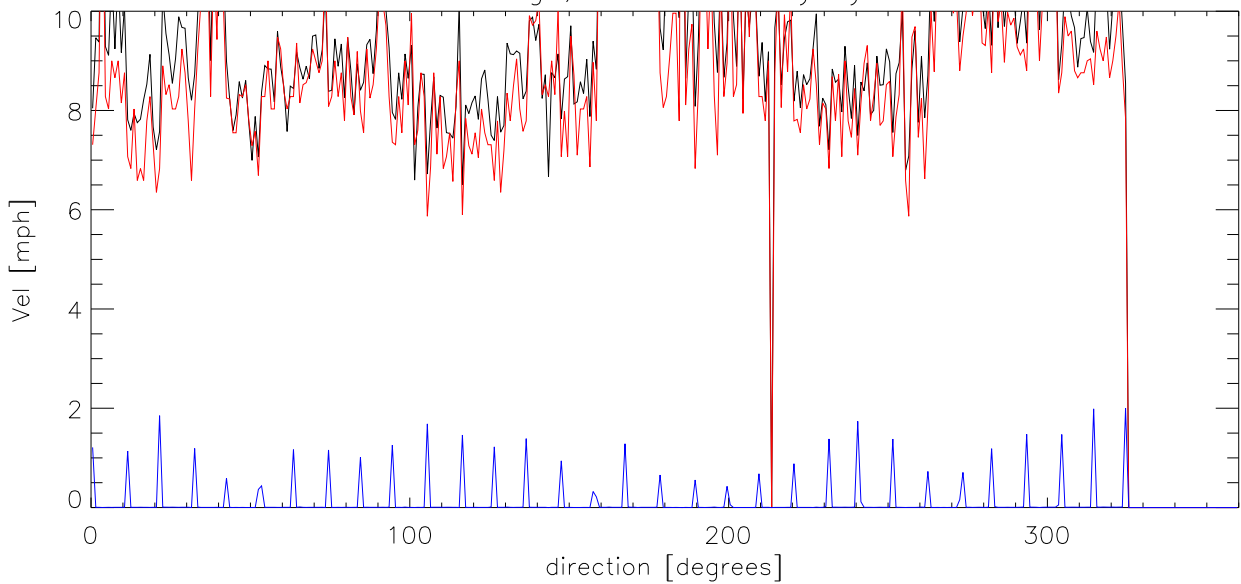
FEB18 Average, median velocity by direction
