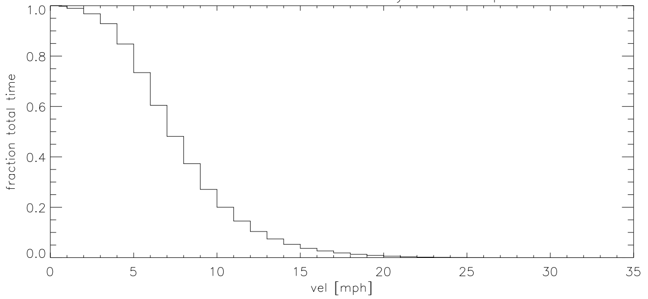
FEB18 Fraction of time wind velocity exceeds specified vel (blowup)
