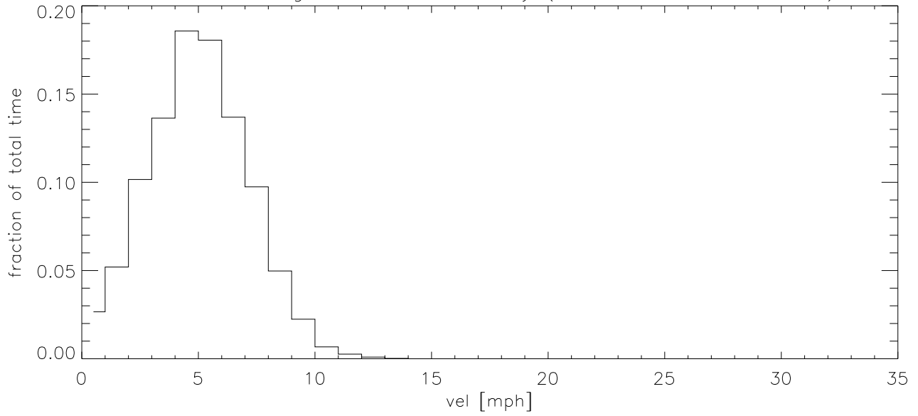
DEC17 Fraction of time wind velocity exceeds specified vel
