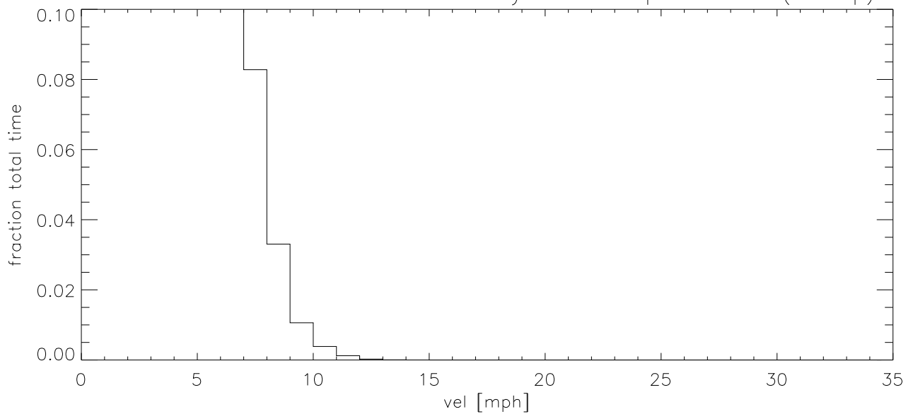
DEC17 Fraction of time wind velocity exceeds specified vel (blowup)
