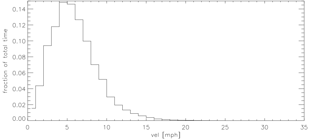
JUN16 Fraction of time wind velocity exceeds specified vel
