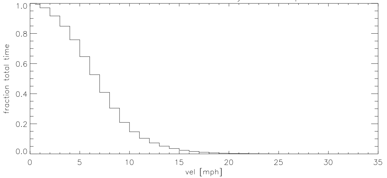
MAR16 Fraction of time wind velocity exceeds specified vel (blowup)
