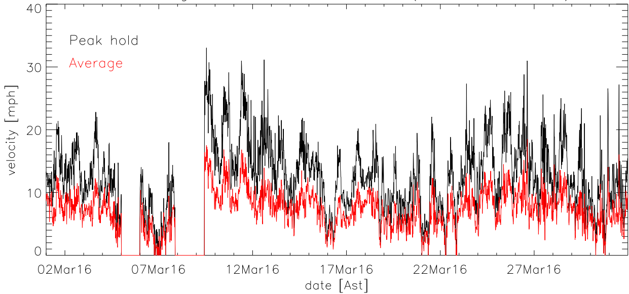
MAR16 Average, median velocity by hour of day
