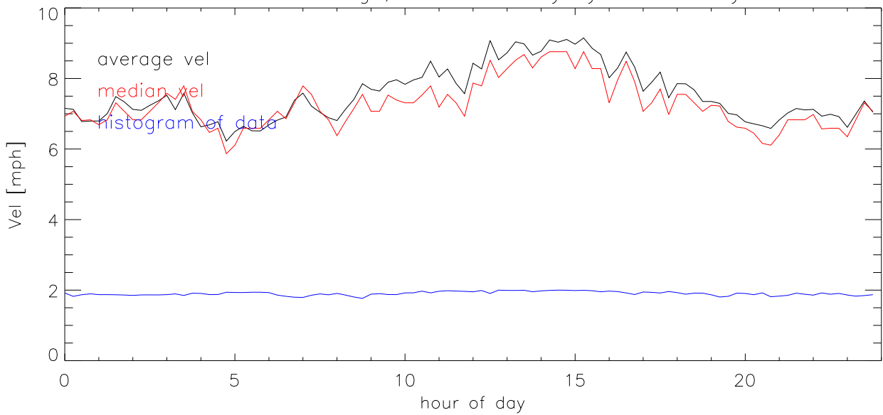
MAR16 Average, median velocity by direction
