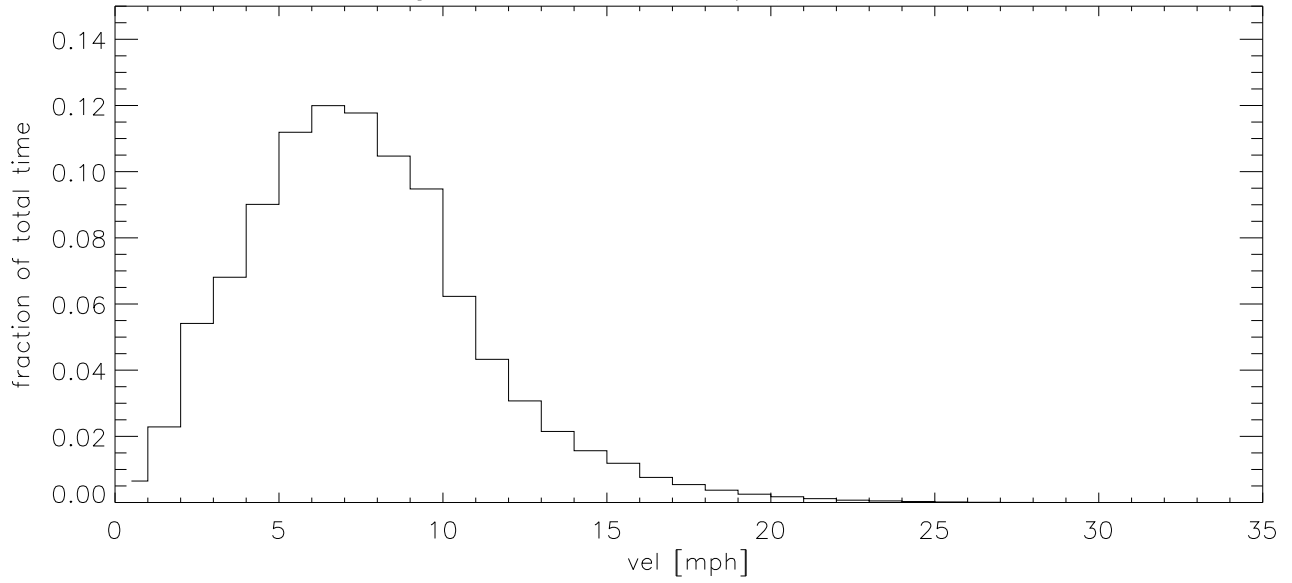
MAR16 Fraction of time wind velocity exceeds specified vel
