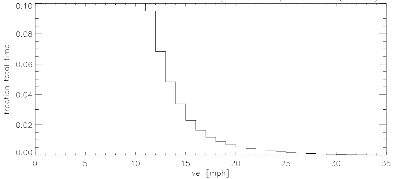
AUG15 Fraction of time wind velocity exceeds specified vel (blowup)
