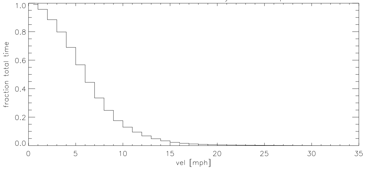
AUG15 Fraction of time wind velocity exceeds specified vel (blowup)
