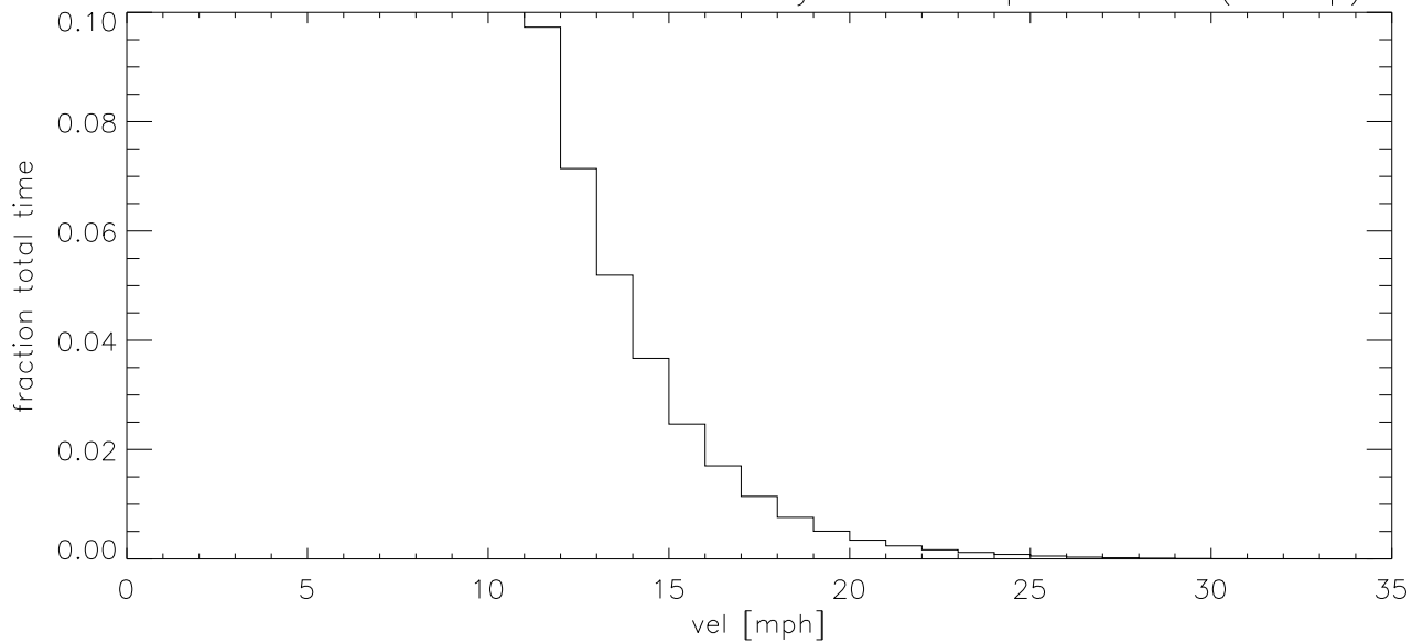
APR15 Fraction of time wind velocity exceeds specified vel (blowup)
