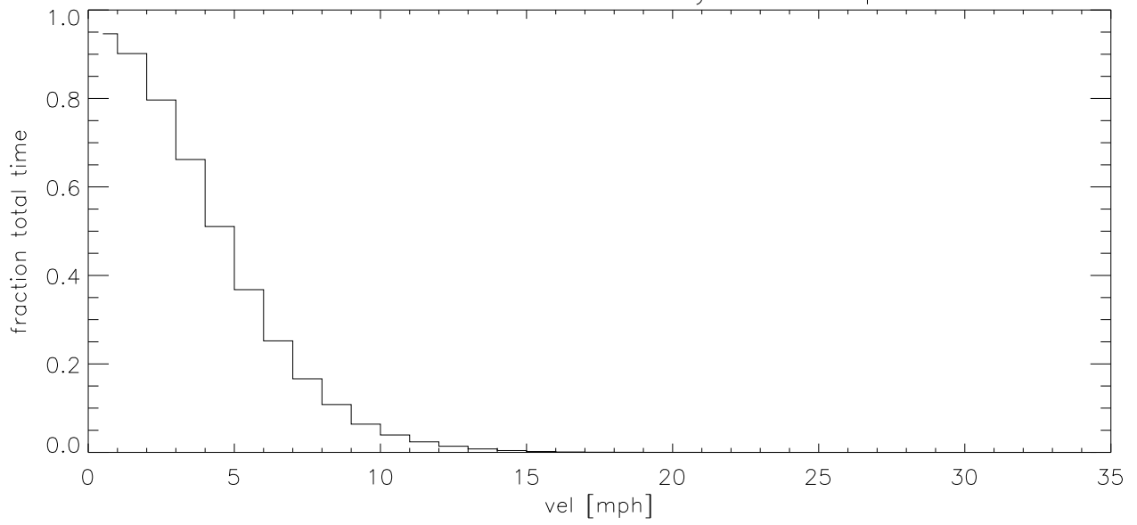
OCT14 Fraction of time wind velocity exceeds specified vel (blowup)
