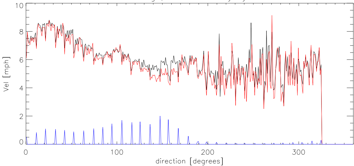
OCT14 Average, median velocity by direction
