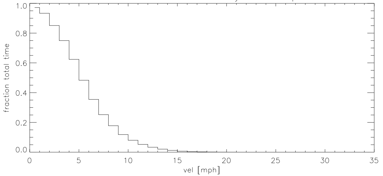
MAR14 Fraction of time wind velocity exceeds specified vel (blowup)
