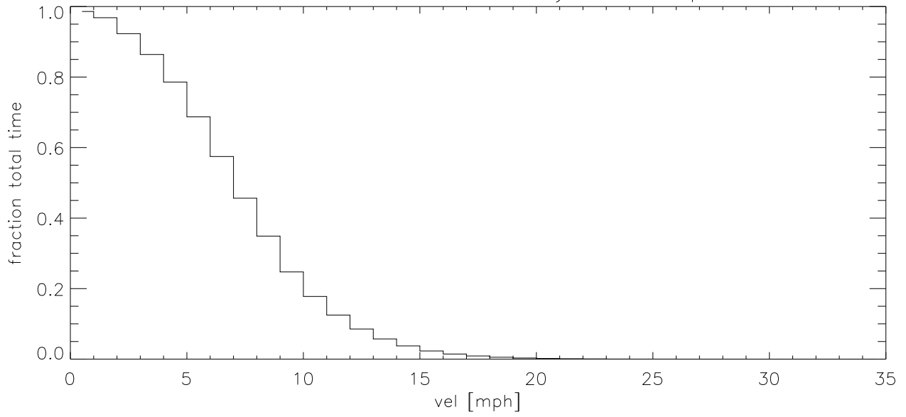
DEC13 Fraction of time wind velocity exceeds specified vel (blowup)
