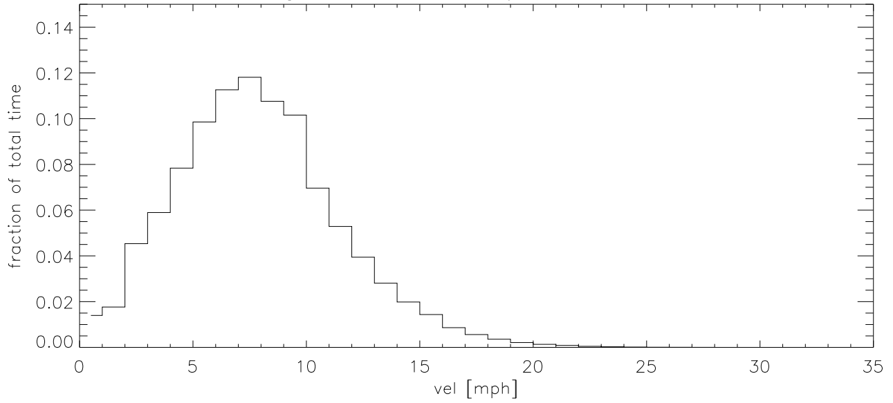
DEC13 Fraction of time wind velocity exceeds specified vel
