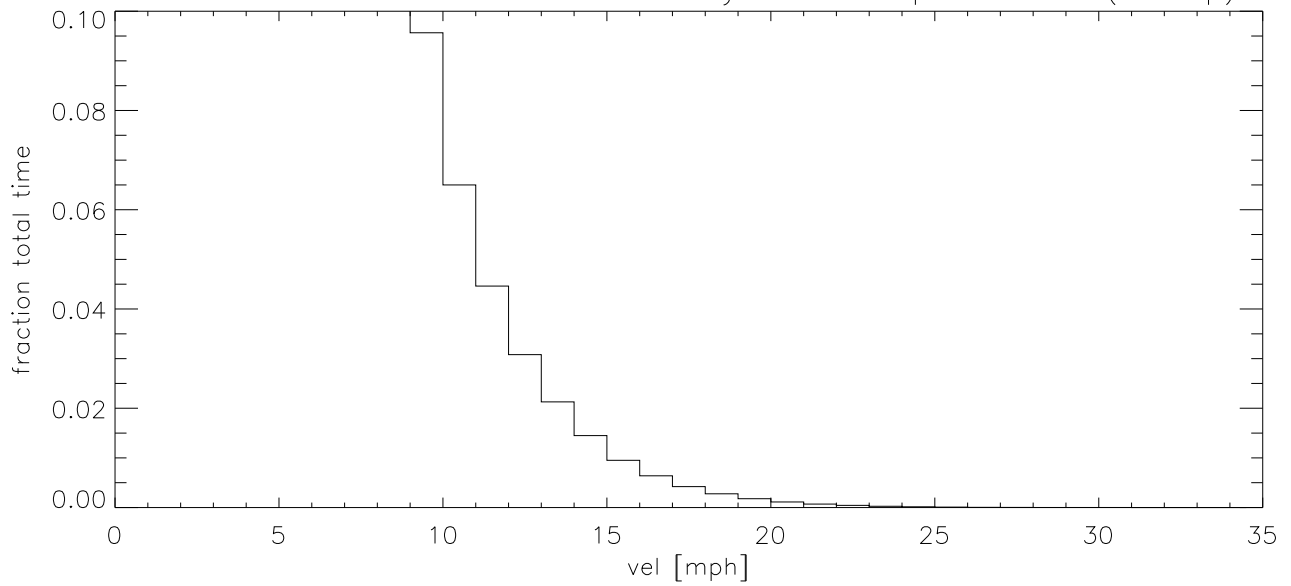
SEP13 Fraction of time wind velocity exceeds specified vel (blowup)
