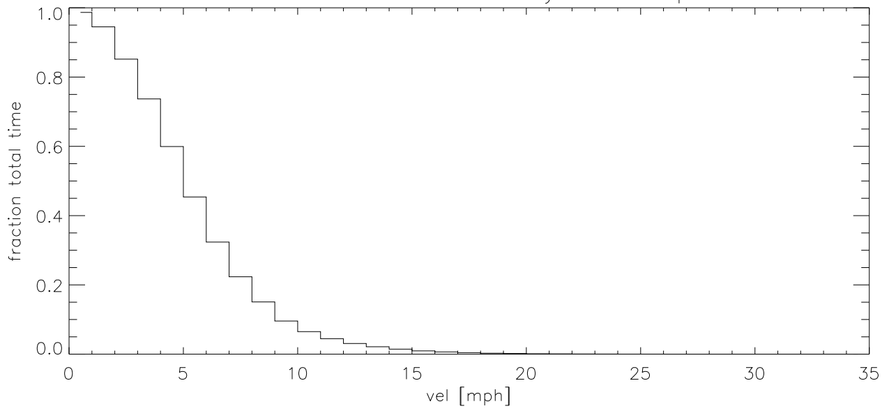
SEP13 Fraction of time wind velocity exceeds specified vel (blowup)
