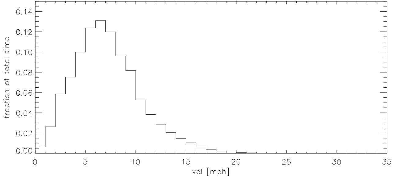
APR13 Fraction of time wind velocity exceeds specified vel
