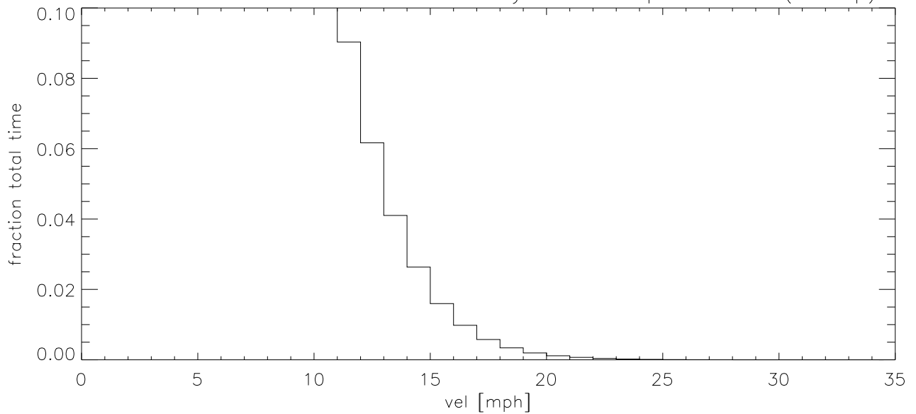
APR13 Fraction of time wind velocity exceeds specified vel (blowup)
