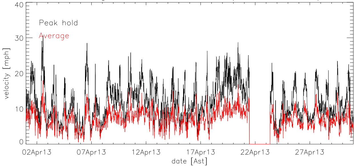
APR13 Average,median velocity by hour of day
