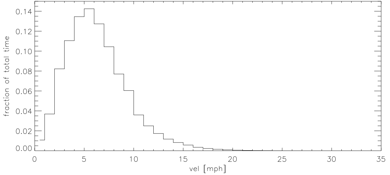
OCT12 Fraction of time wind velocity exceeds specified vel
