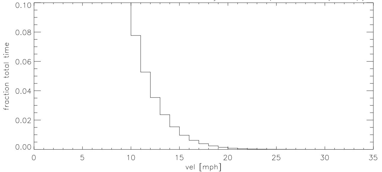
OCT12 Fraction of time wind velocity exceeds specified vel (blowup)
