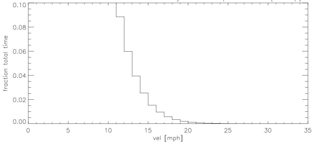
MAR12 Fraction of time wind velocity exceeds specified vel (blowup)
