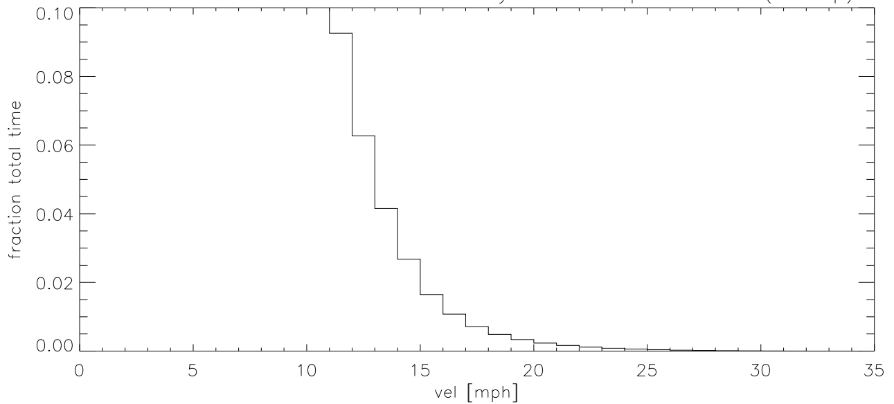
JUL10 Fraction of time wind velocity exceeds specified vel (blowup)
