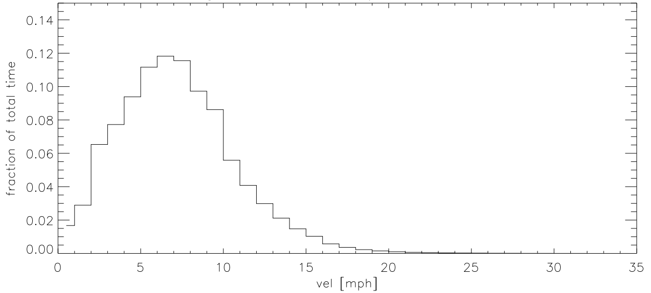
JUL10 Fraction of time wind velocity exceeds specified vel
