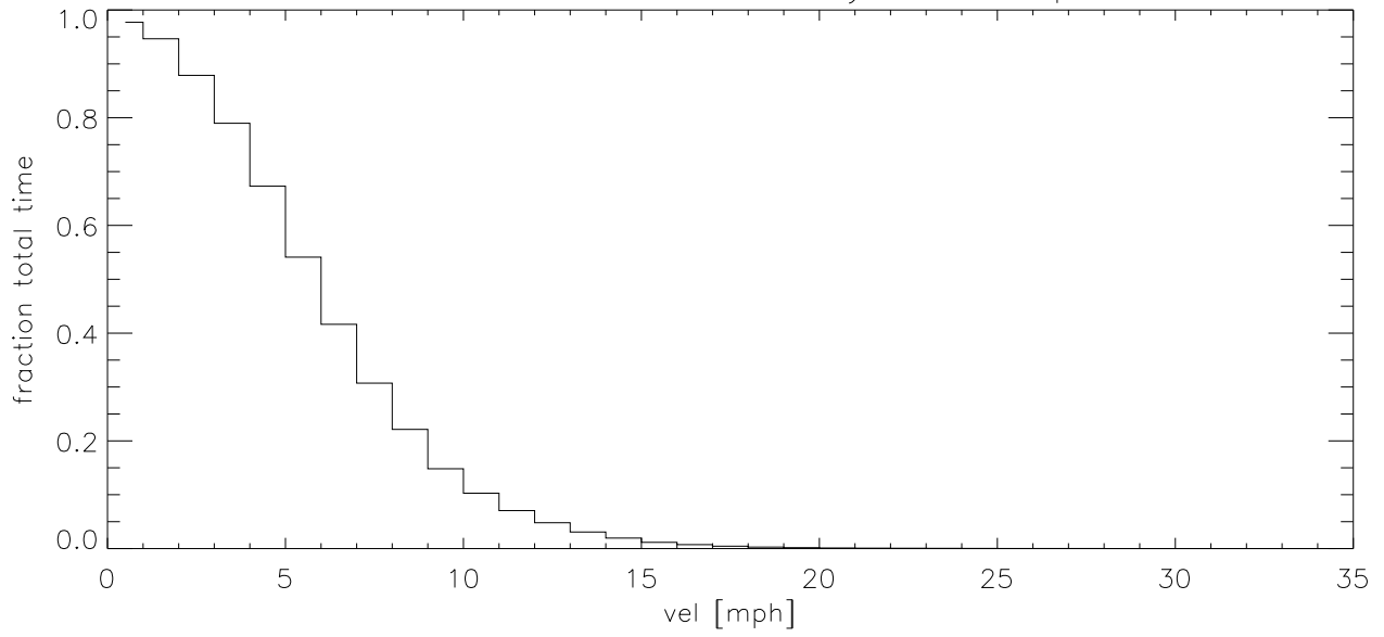
MAY10 Fraction of time wind velocity exceeds specified vel (blowup)
