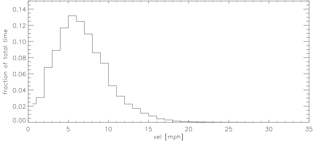
MAY10 Fraction of time wind velocity exceeds specified vel
