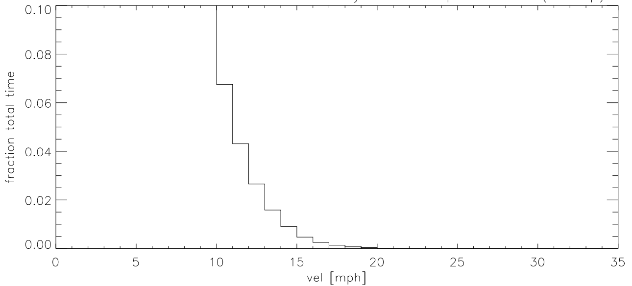
MAY09 Fraction of time wind velocity exceeds specified vel (blowup)
