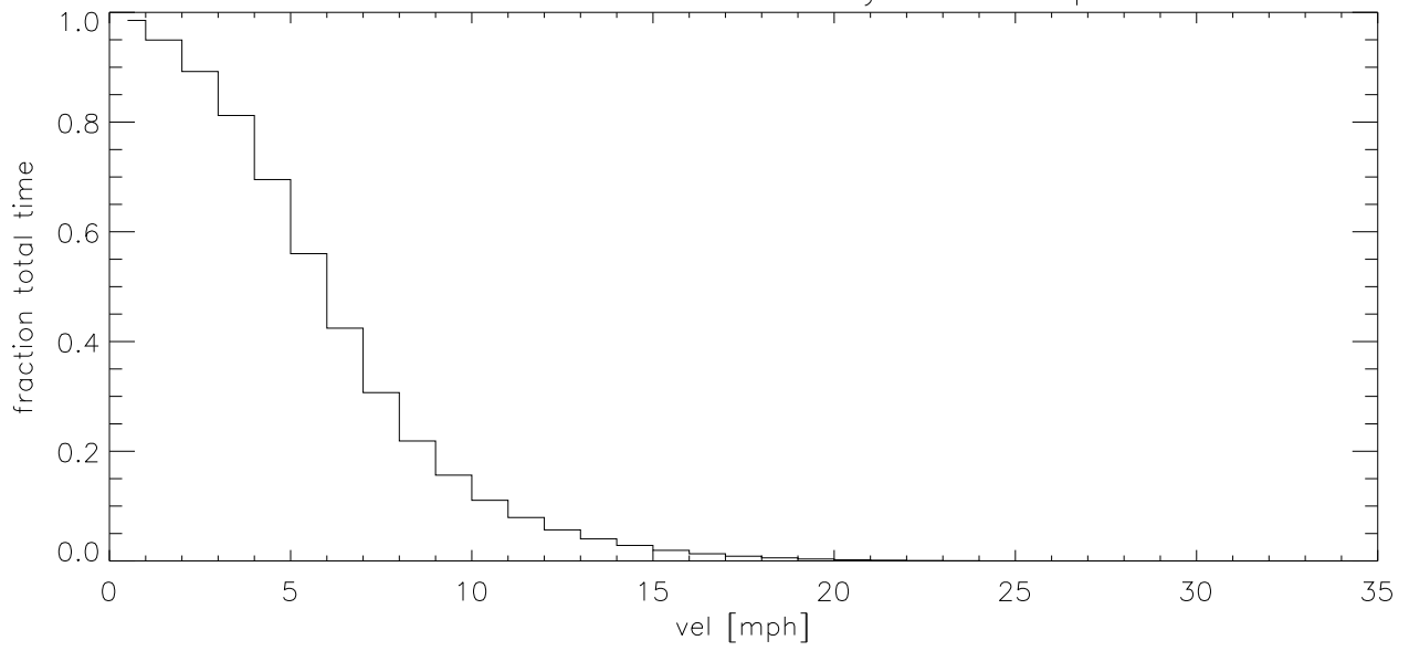
AUG07 Fraction of time wind velocity exceeds specified vel (blowup)
