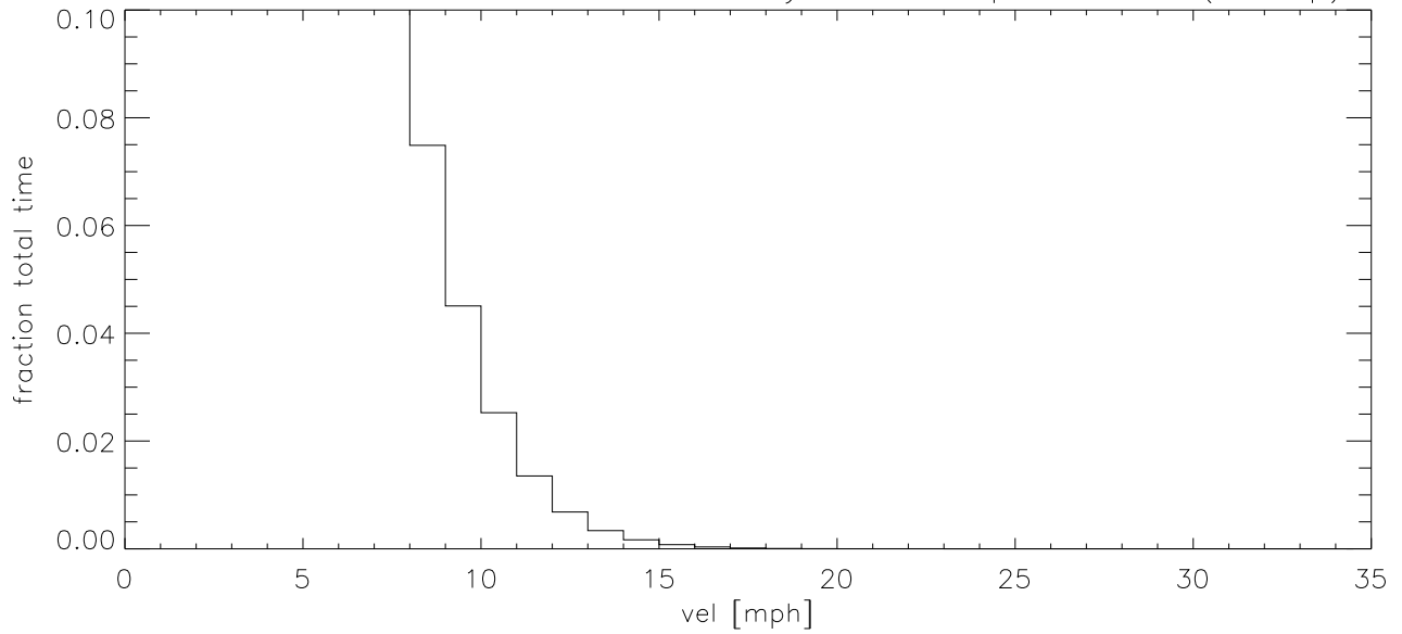
MAY07 Fraction of time wind velocity exceeds specified vel (blowup)
