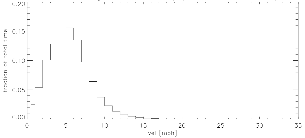
SEP06 Fraction of time wind velocity exceeds specified vel
