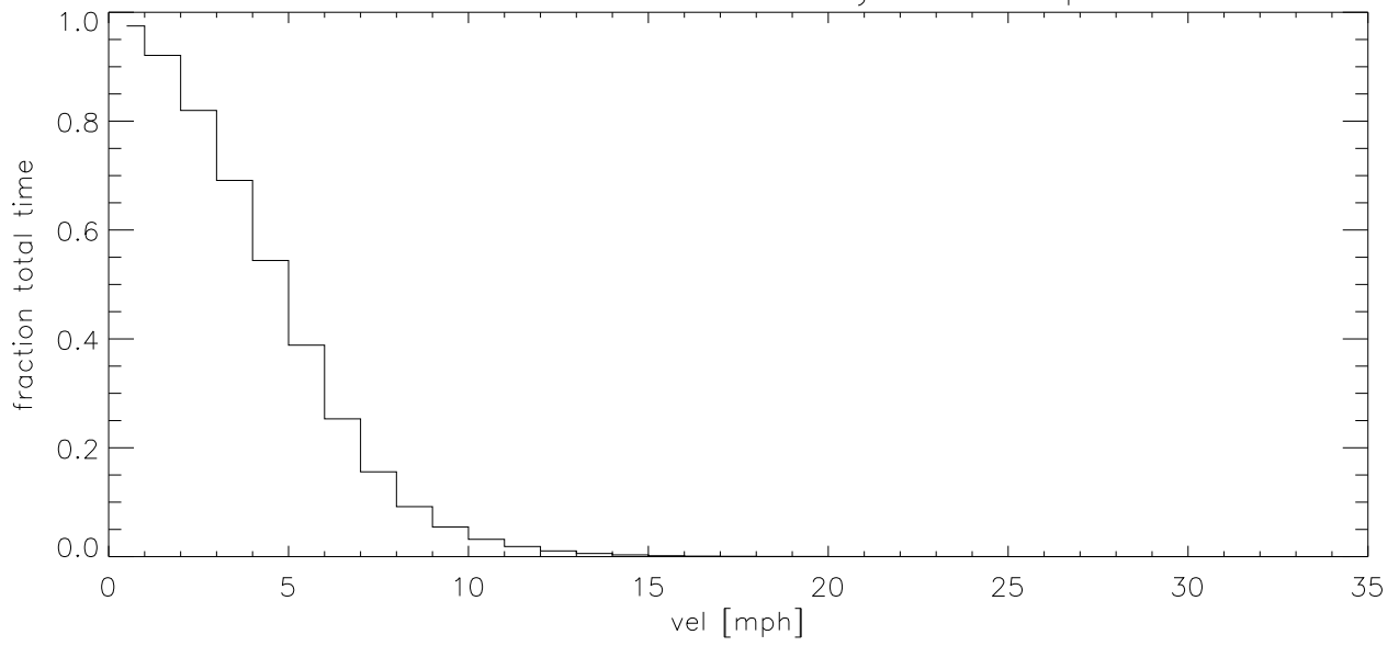
SEP06 Fraction of time wind velocity exceeds specified vel (blowup)
