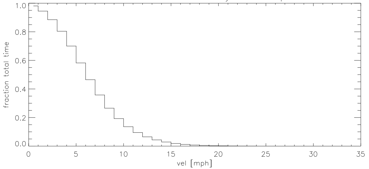
JAN06 Fraction of time wind velocity exceeds specified vel (blowup)
