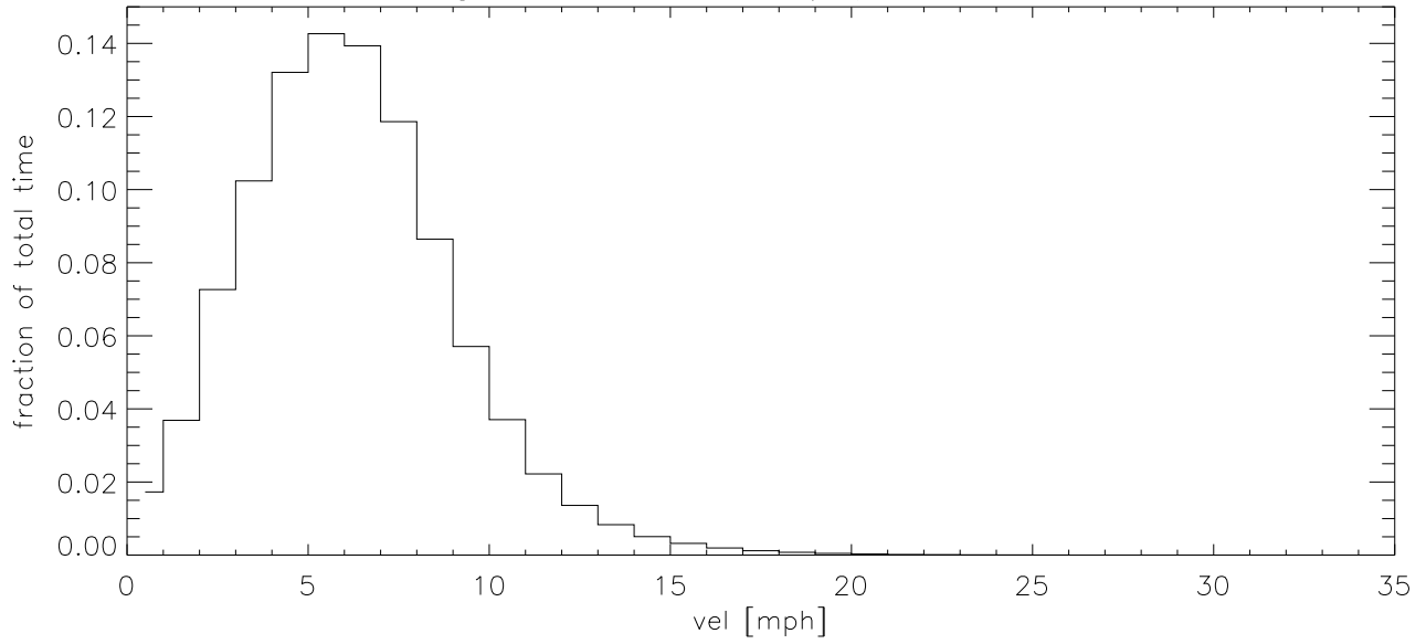
DEC05 Fraction of time wind velocity exceeds specified vel
