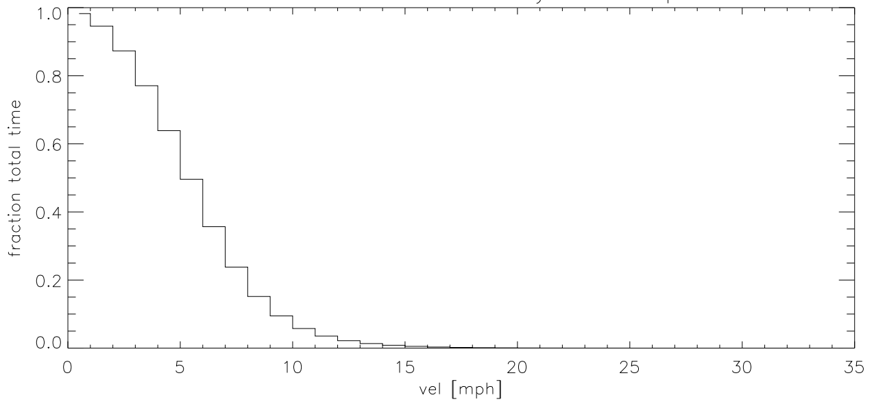
DEC05 Fraction of time wind velocity exceeds specified vel (blowup)
