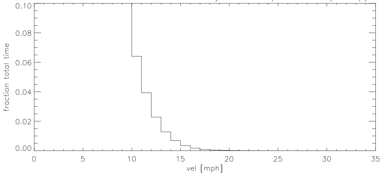
AUG03 Fraction of time wind velocity exceeds specified vel (blowup)
