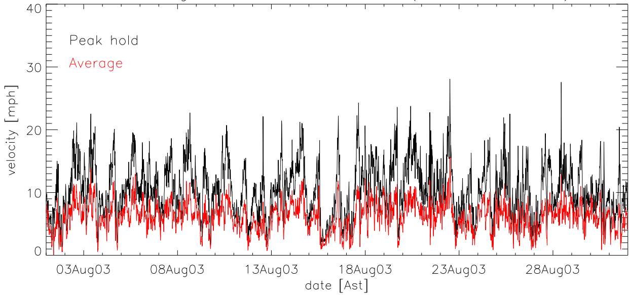
AUG03 Average, median velocity by hour of day
