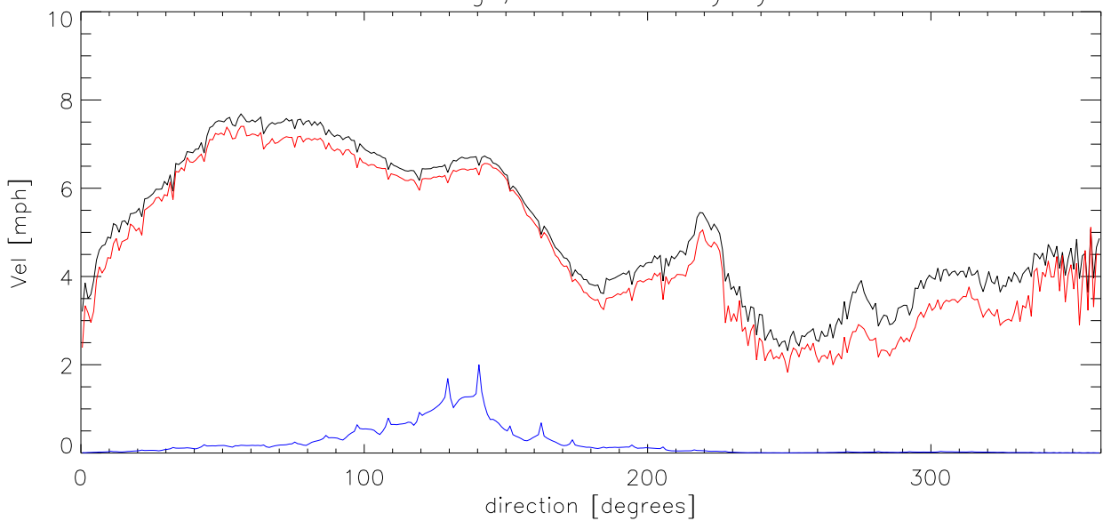
AUG03 Average, median velocity by direction
