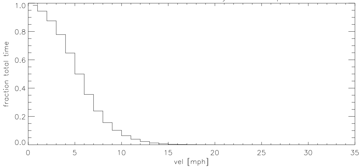
AUG03 Fraction of time wind velocity exceeds specified vel (blowup)
