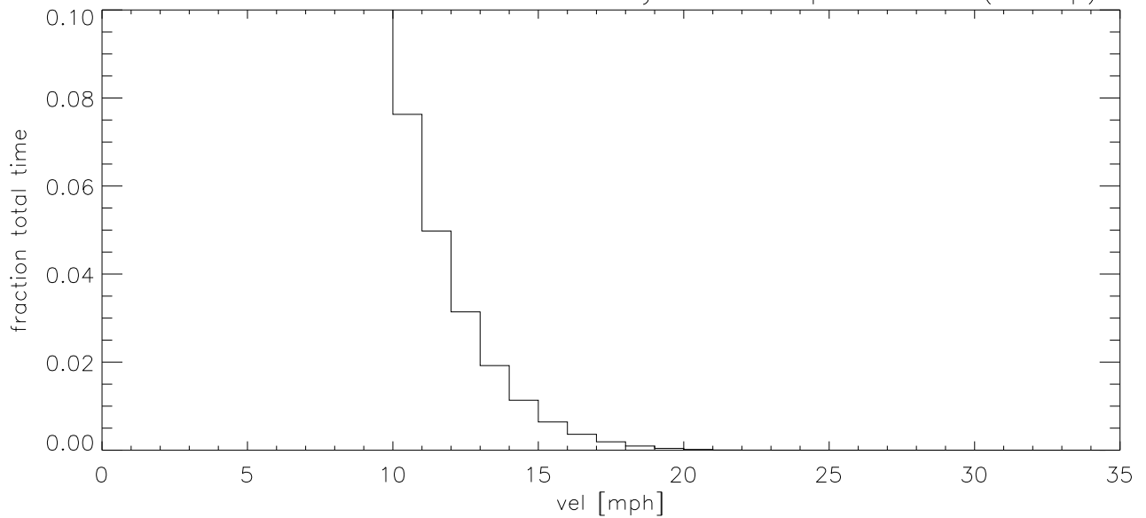
MAR03 Fraction of time wind velocity exceeds specified vel (blowup)
