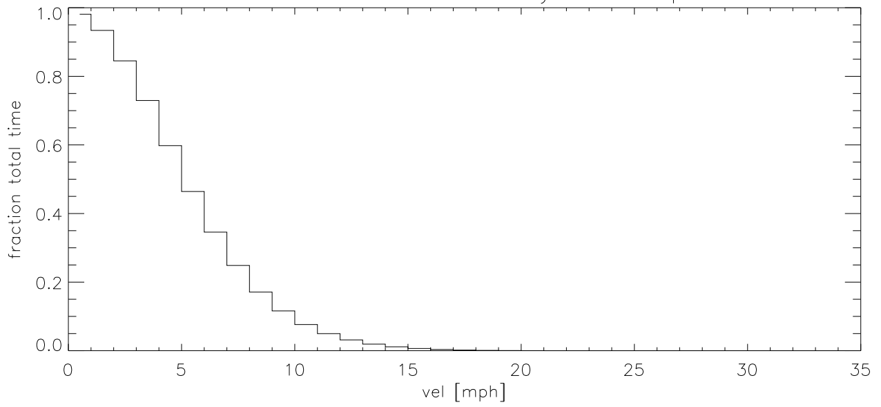
MAR03 Fraction of time wind velocity exceeds specified vel (blowup)
