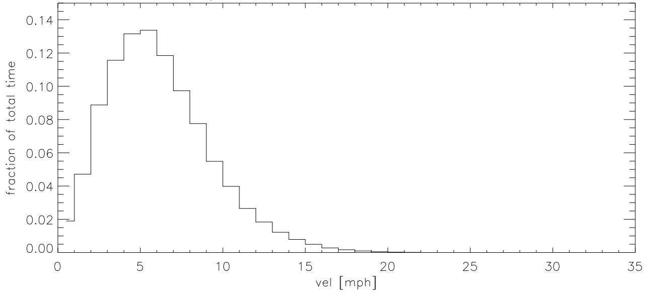
MAR03 Fraction of time wind velocity exceeds specified vel
