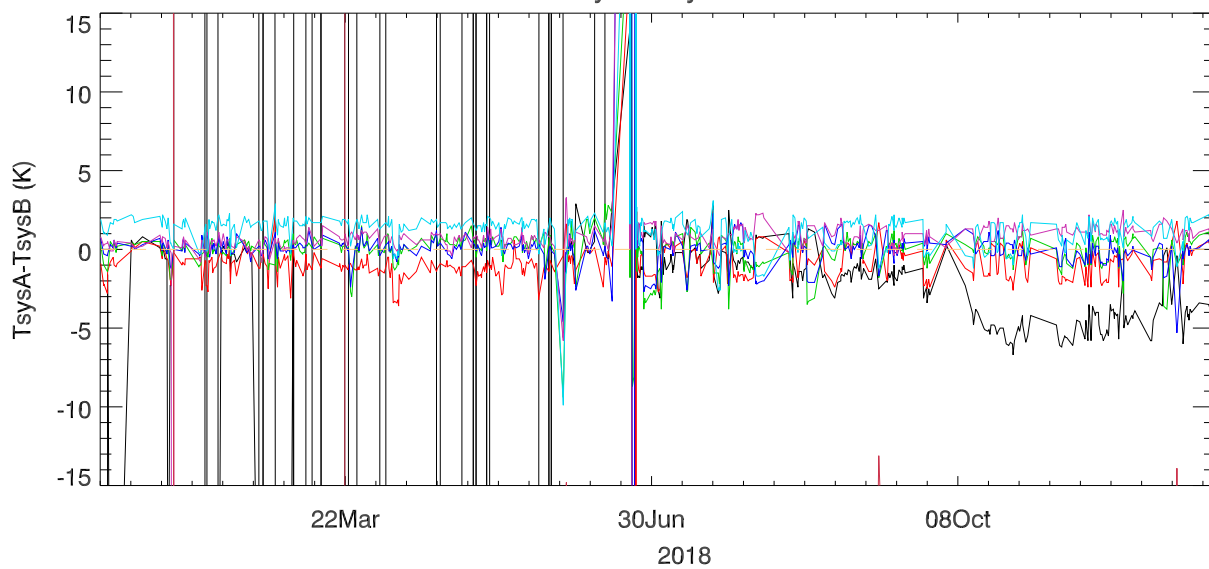
alfa TsysA-TsysB 2018
