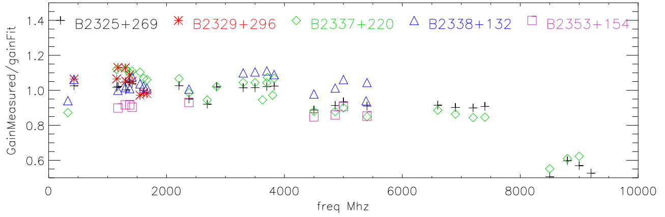
median gain ratio (measured/fit) vs freq jan04 thru sep17
