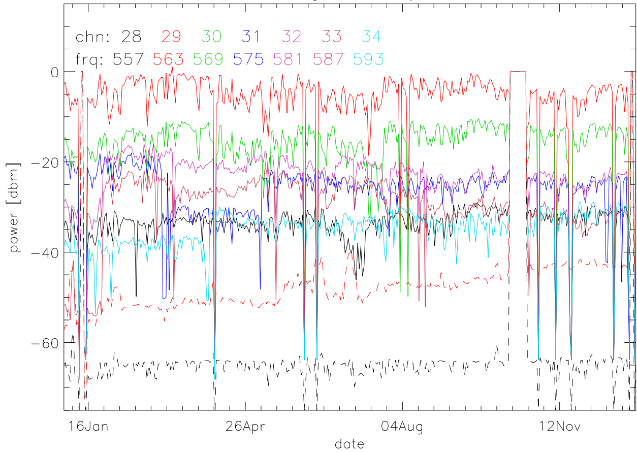
TV stations hilltopMonitoring 2019:daily min. 550Mhz RfiBand
