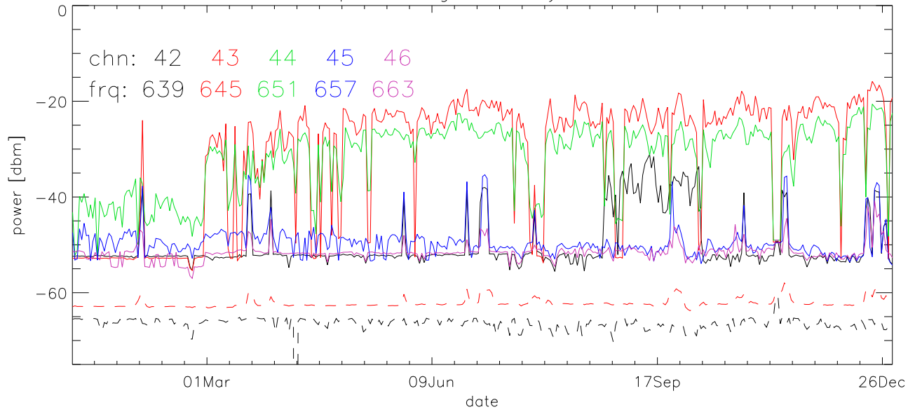
TV stations hilltopMonitoring 2003:daily min. 725Mhz RfiBand
