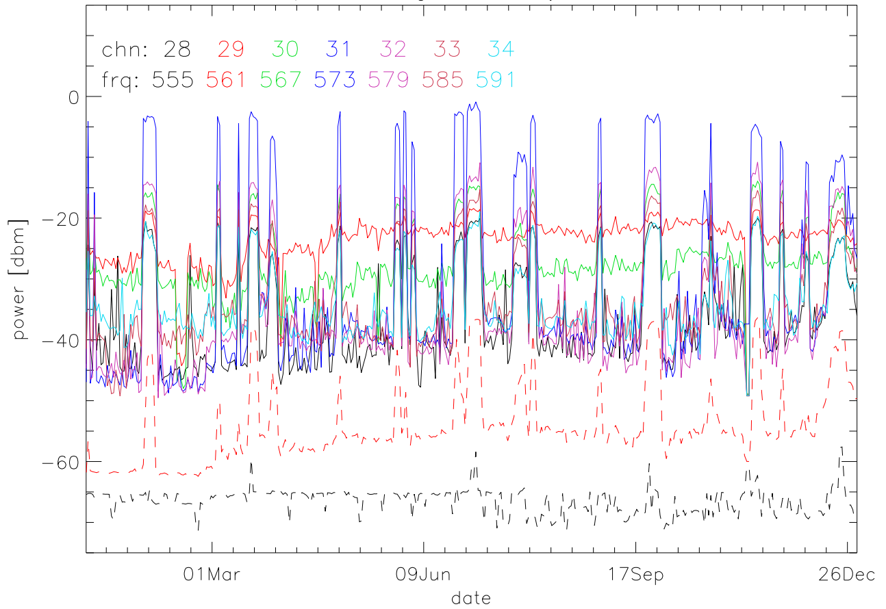
TV stations hilltopMonitoring 2003:daily max. 550Mhz RfiBand
