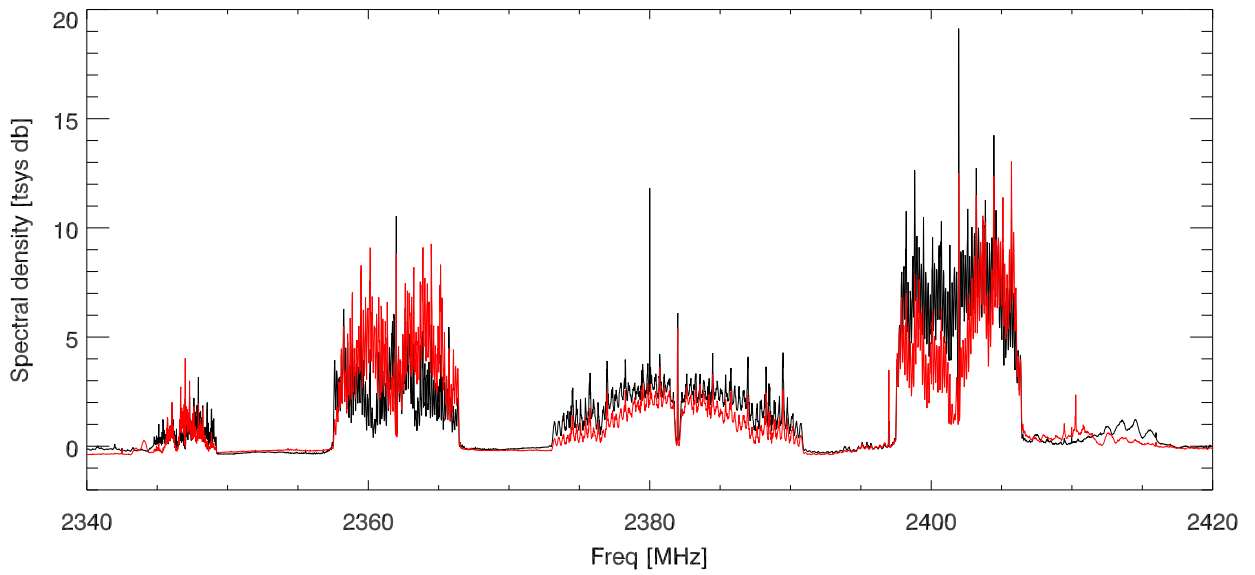
sbn 10GhzUpConverter IF, skyCfr:2385MHz. A/D cfr:2385MHz
