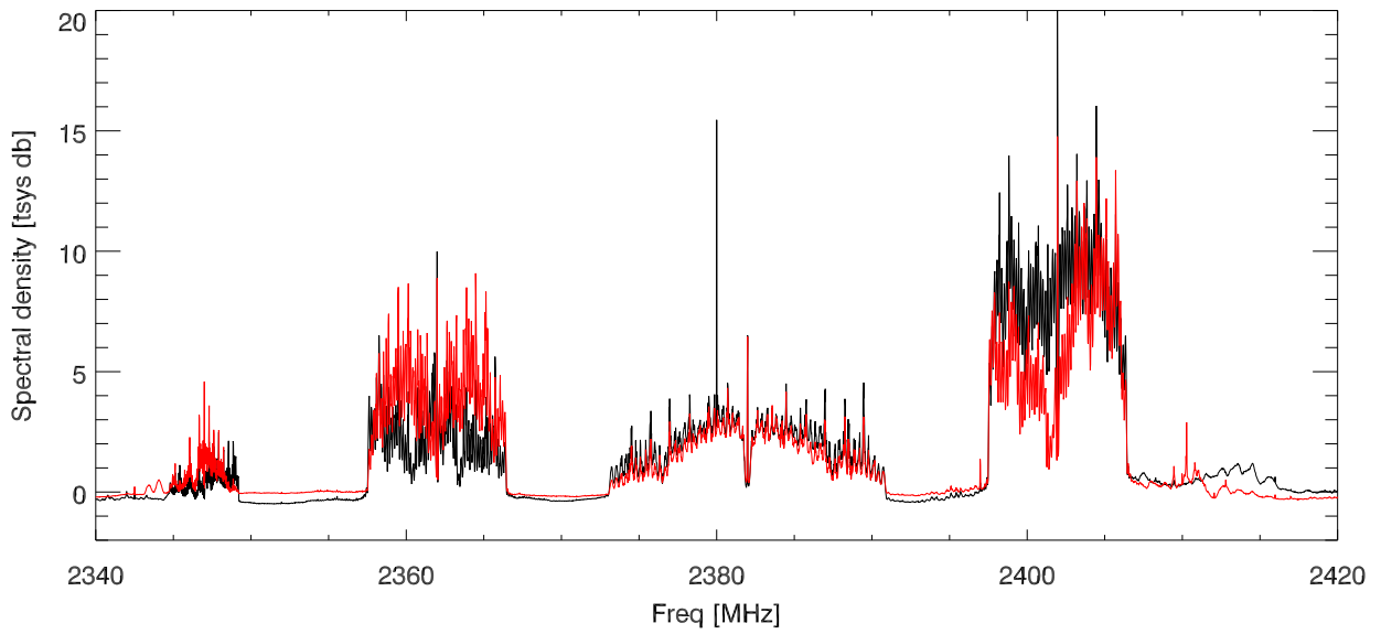
05sep15: 2380 MHz rfi. sbn 750 IF, skyCFR:2380MHz,A/D cfr:2380MHz
