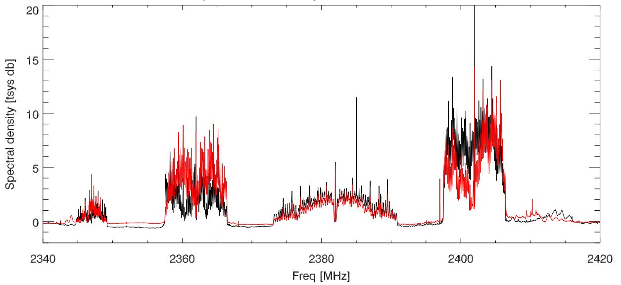
sbw 10GhzUpConverter IF, skyCfr:2360MHz. A/D cfr:2360MHz
