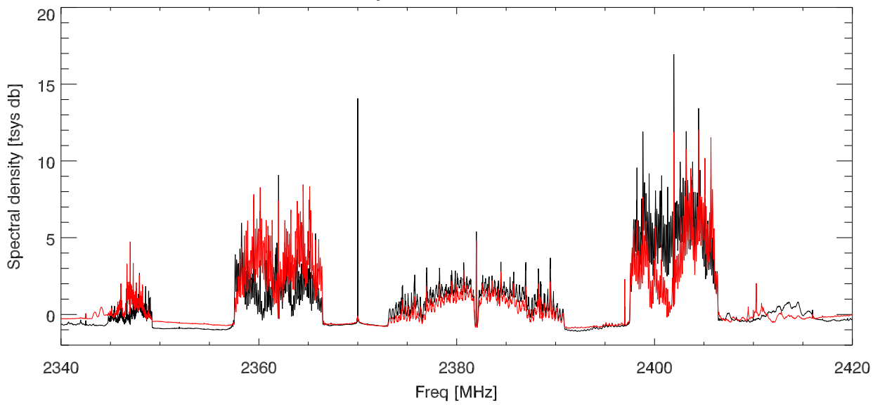
sbn 10GhzUpConverter IF, skyCfr:2380MHz, A/D cfr:2380MHz
