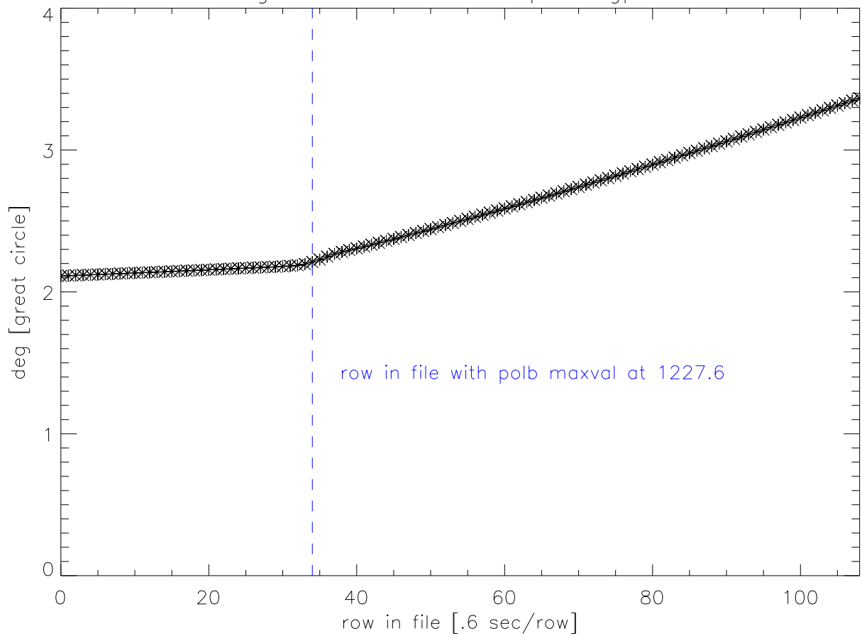
angular distance telescope to gps 22
